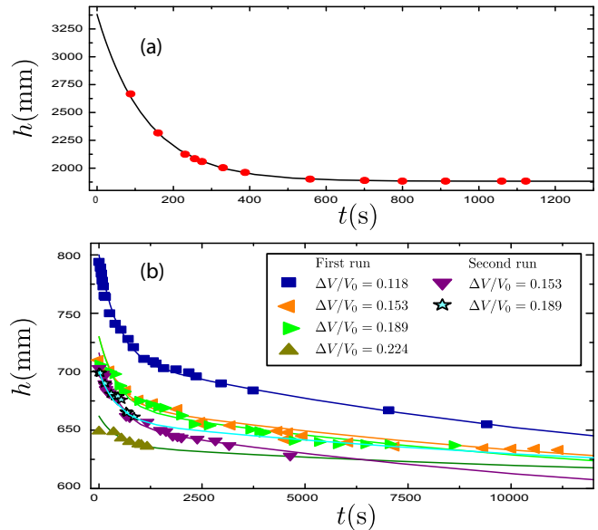
Fig. 5. "Slow devices": Time evolution of the slump h of water level in the manometer. (a) Monoexponential relaxation with a characteristic time \tau = 129 s for a ball of radius R = 22.5 mm and relative thickness d/R = 0.222 ; relative volume variation after stabilization ( i.e. calculated using h_{asymp} in Eq. (1)) \frac{\Delta V_{asymp}}{V_0} = 0.211 . (b) Biexponential relaxation for different values of the volume sucked out from a ball of radius R = 58.7 mm and d/R = 0.097 , during 2 different sequences of deflation. All theoretical curves correspond to a biexponential fit with the same pair of characteristic times ( \tau_1 = 440 s, \tau_2 = 15000 s) and the same proportion p = 0.42 of short-time exponential.
