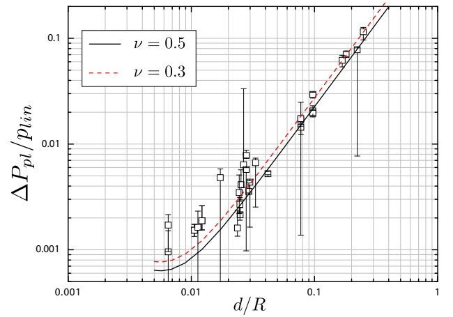
Fig. 9. Squares: values of \Delta P_{pl}/p_{lin} , obtained from deflation curves similar to Fig. 4-b or Fig. 7, where \Delta P_{pl} is the minimum value of the post-buckling regime, normalized by the slope p_{lin} of the pre-buckling linear part. Lines: theoretical values determined using Eq. (14).
