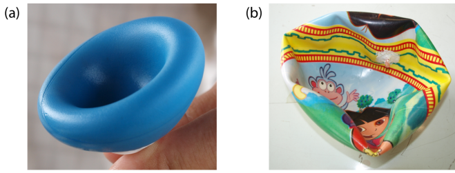
Fig. 2. Elastic shells almost fully deflated; the hemisphere that is curved inward is in contact with the, mainly unchanged, other half of the shell. (a) Thick shell (relative thickness d/R = 0.18 ; external radius R + d/2 = 55.5 mm), in which axisymmetry was conserved throughout the deflation. (b) Thin shell ( d/R = 10.6 \cdot 10^{-3} ; external radius R + d/2 = 190 mm), where radial folds began to develop inside the depression at some point of the deflation process.
