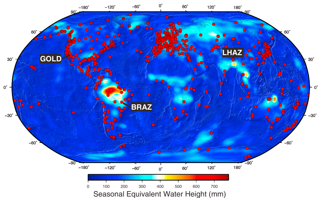
Figure 1. Peak-to-peak surface load variations, expressed in equivalent-water height (in mm), derived from Gravity Recovery and Climate Experiment for the 2002–2012 period and corrected from detectable coseismic and postseismic contributions. Red dots show the locations of the continuous Global Positioning System stations used in this study. LHAZ, GOLD, and BRAZ are highlighted because time series for these three stations are shown as examples later on.
