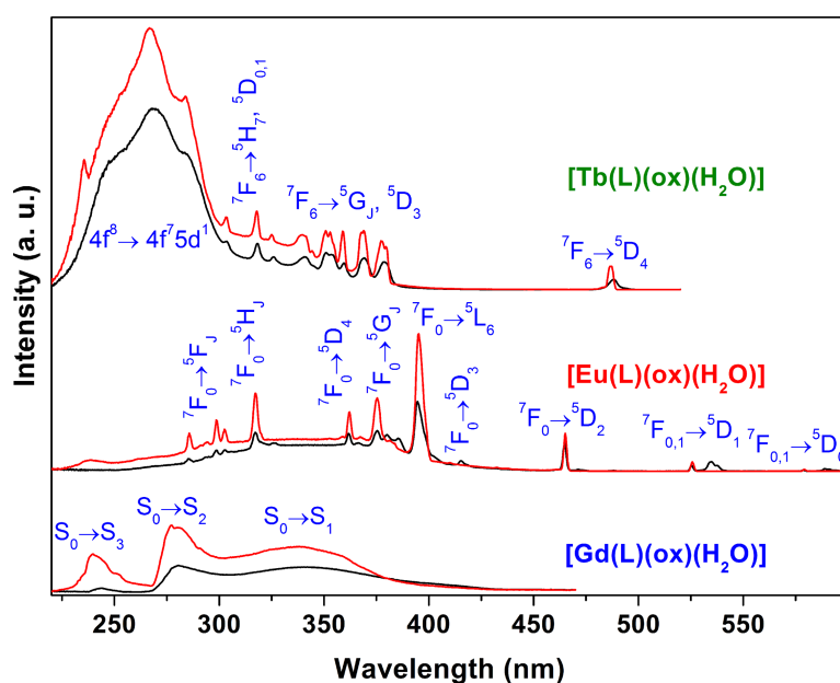
Figure 4: Excitation spectra of [\text{Gd}(\text{L})(\text{ox})(\text{H}_2\text{O})] ( \lambda_{\text{Em}} = 520 \text{ nm} ), [\text{Eu}(\text{L})(\text{ox})(\text{H}_2\text{O})] ( \lambda_{\text{Em}} = 619.6 \text{ nm} ) and [\text{Tb}(\text{L})(\text{ox})(\text{H}_2\text{O})] ( \lambda_{\text{Em}} = 542 \text{ nm} ) recorded at 297 K (black lines) and 12 K (red lines). The intensity is only comparable for the variation of the temperature in each compound.
