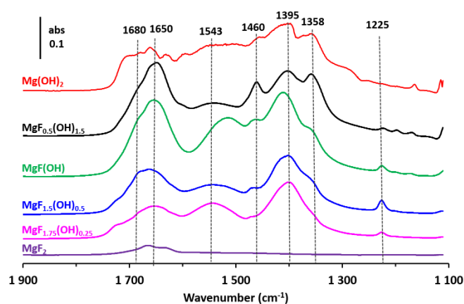
Fig. 4 Difference of IR spectra obtained after CO_2 adsorption at 50\text{ }^\circ\text{C} and after activation at 90\text{ }^\circ\text{C} under vacuum of MgF_{2-x}(OH)_x samples with 0 \leq x \leq 2
