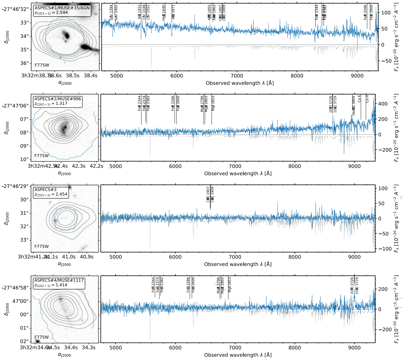
Figure 13. MUSE spectroscopy of the ASPECS-LP sources. Left: HST /F775W cutout. The colored contour(s) mark the region of the spectral extraction(s), defined by convolving the MUSE PSF with the HST segmentation map (see Inami et al. 2017 for details), or a fixed 0''.8 aperture (in the case of a new extraction; #3, #7, #9, #13). The black contours indicate the CO emission from \pm[3, \dots, 11]\sigma in steps of 2\sigma . Right: MUSE spectrum ( 1.5 \text{ Å} Gaussian smoothing) extracted over the marked region. The 1\sigma uncertainty on the spectrum is shown by the gray line in the direction of negative flux (for clarity), and is largest around skylines. The (expected) positions of different spectral features are annotated; this does not indicate that the feature is also detected. Spectra and lines of nearby or blended sources are shown in red.
