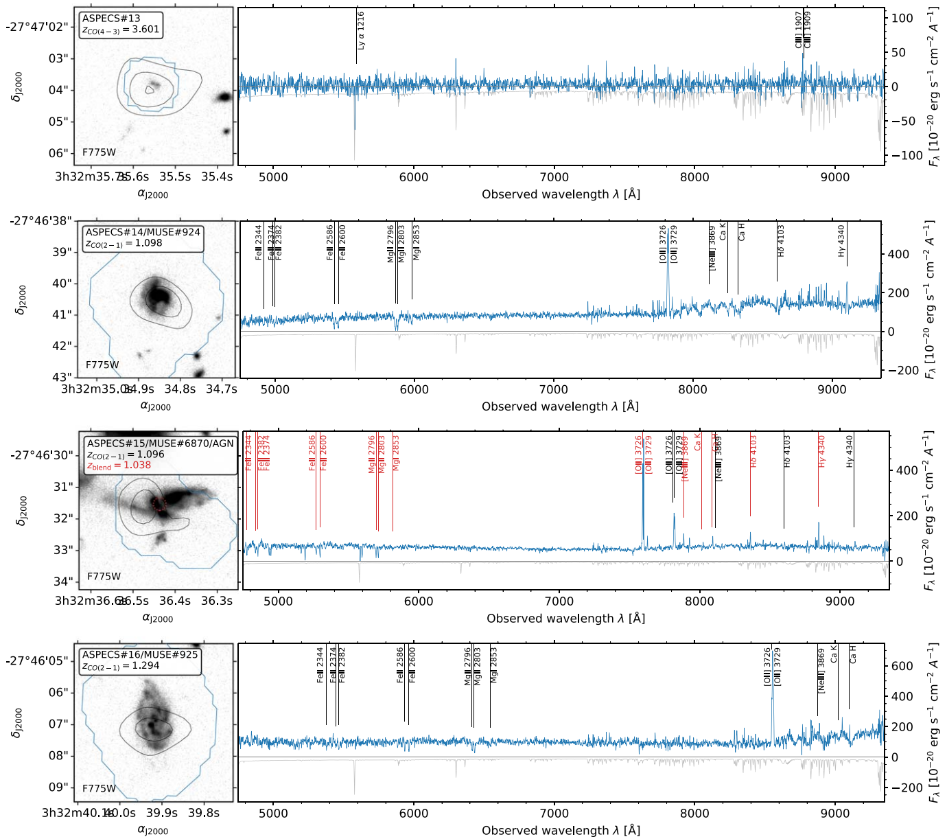
Figure 16. Continuation of Figure 13. The spectrum of ASPECS-LP.3mm.15 is severely blended. We have highlighted the strongest blended features (from a foreground source at z = 1.038 ) in red.
