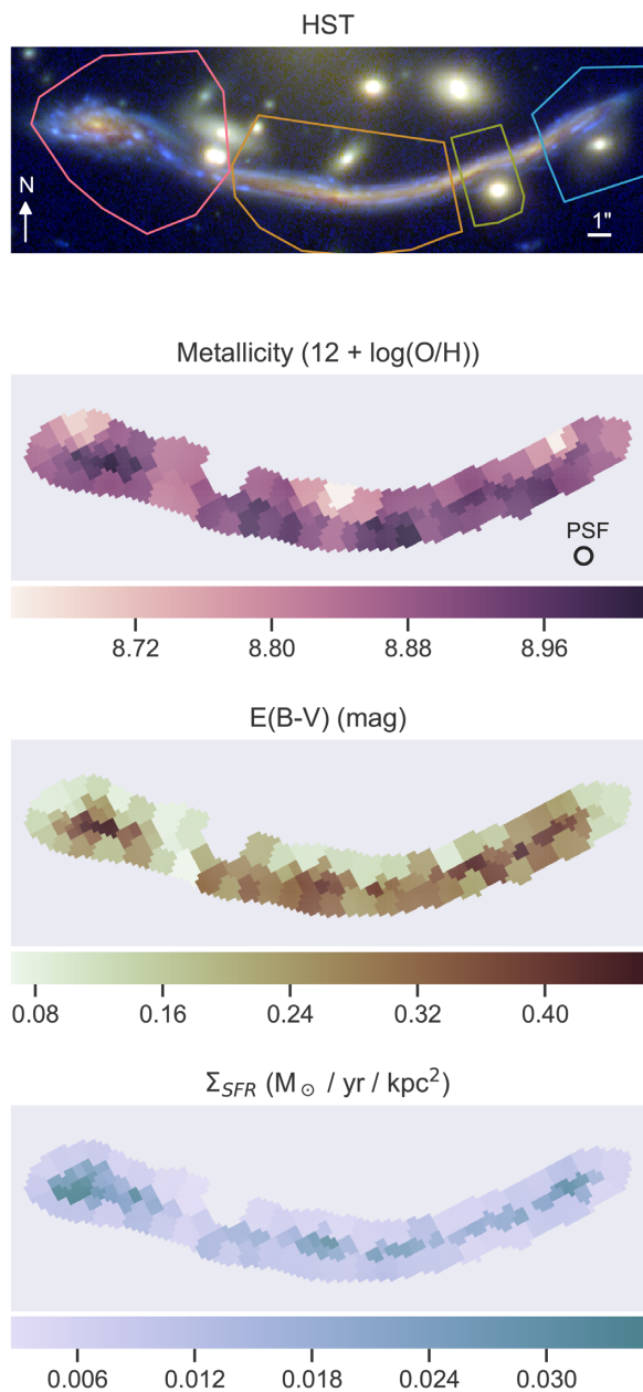
Figure 4. A370-sys1 in the image plane. Top panel: HST composite image with filters F160W, F814W, and F435W. Contours correspond to the different multiple images, with the complete image in pink. Lower panels: metallicity, extinction, and SFR surface density maps, from top to bottom, each colour coded in a different colour scheme. The FWHM of the PSF plotted in the lower right-hand corner of the bottom panel. All images have the same physical size and orientation.
