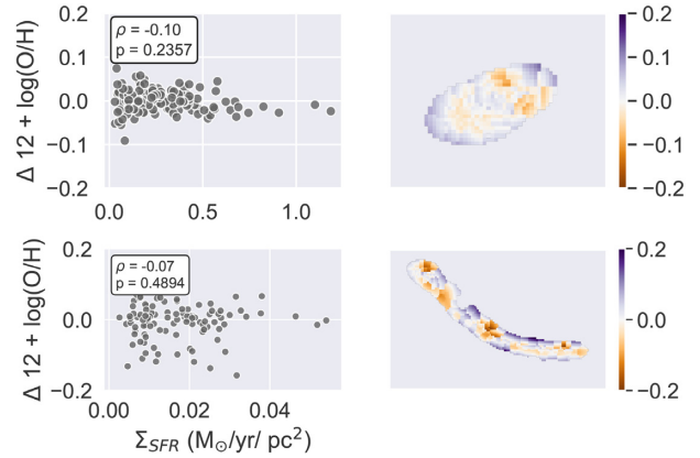
Figure 10. Metallicity gradient residuals. Top: AS1063-arc. Bottom: A370-sys1. Left: residuals after subtracting fitted gradient versus star formation rate density. The Spearman rank-order correlation coefficient and respective p value calculated for each of the two properties plotted are shown in the top left-hand corner of each plot. Right: 2D residuals map.
