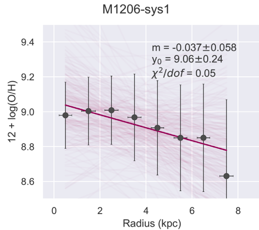
Figure 9. M1206-sys1 radial variation of metallicity. The data points correspond to averages within annuli. The fit was performed with the LINMIX package. The pink lines are multiple realizations of the fit. The thick line corresponds to the average of all these possible slopes, and we plot its slope ( m ) and intercept ( y_0 ) and uncertainties in the top right-hand corner.
