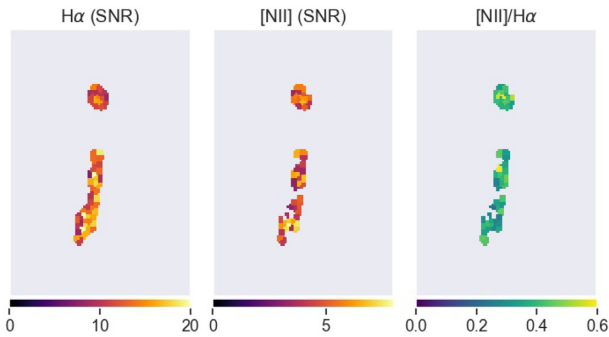
Figure A3. M1206-sys1 signal-to-noise ratios maps of H\alpha and [N\text{II}]\lambda 6585 (left-hand and middle panels) and ratio of the two (right-hand panel).
