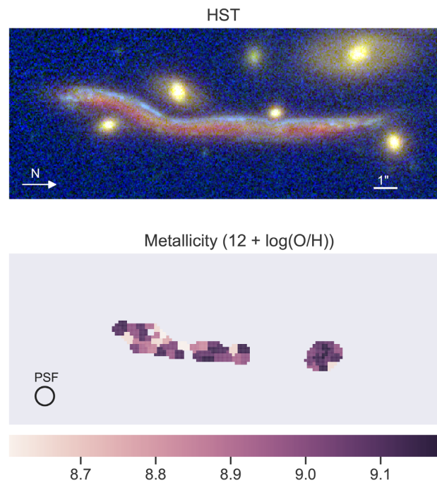
Figure 5. M1206-sys1 in the image plane. Top panel: HST composite image with filters F160W, F814W, and F43W5W. Bottom panel: metallicity derived from H\alpha and [N\ II]\ \lambda 6585 . The FWHM of the PSF is plotted in the lower left-hand corner of the bottom panel.
