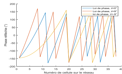
Figure 5. Lois de phase.
