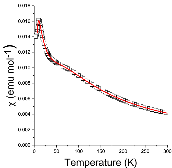
Figure 7. \chi = f(T) curve at 5000 G for compound 1 (open squares: experimental points, full red line: best fit).
