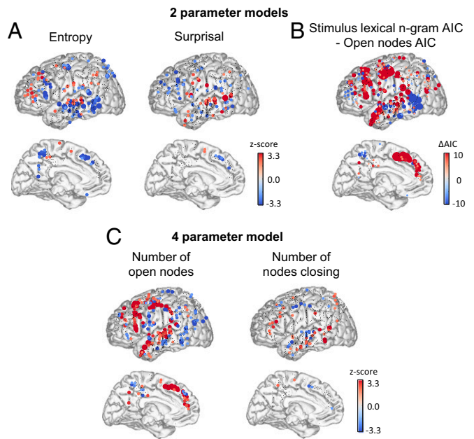
Fig. 4. Stimulus n-gram lexical transition probability model. (A) Stimulus n-gram lexical entropy and surprisal coefficient z scores. Plots show the z score for each electrode in the dataset of the coefficient for entropy (Left) and surprisal (Right) resulting from a model including both parameters in a multiple regression along with other control factors. (B) Comparison of model fit to the open-nodes model. Plots show the AIC differences between the two-parameter stimulus lexical n-gram model and the open-nodes model shown in Fig. 2 C and E. Lower AIC values indicate a better model fit, and therefore, red dots indicate a better fit of the open-nodes model at that electrode site. (C) Representation of the number of open nodes and the number of nodes closing in a four-parameter model also incorporating lexical surprisal and entropy as additional control variables. The strength and significance of the effects of open nodes are not much affected by the addition of the stimulus n-gram lexical entropy and surprisal values. SI Appendix, Table S5 shows the results of significance tests across electrodes and across subjects for each ROI.
