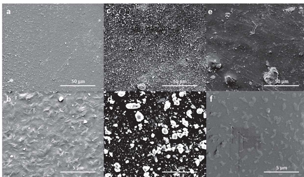
Fig. 2. SEM images of (a,b) CS-PEG400-GLY-20%, (c,d) UV5 and (e,f) P4.
