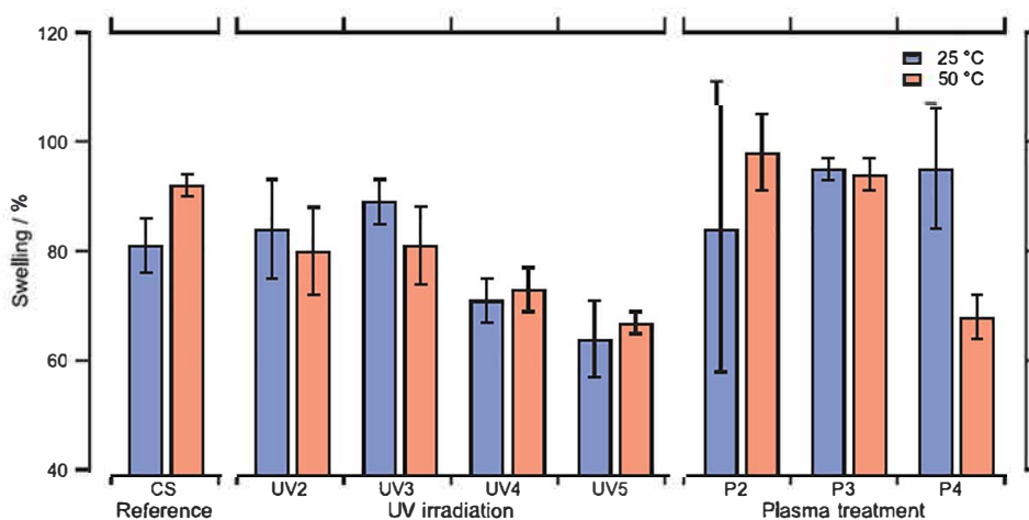
Fig. 3. Swelling properties in an aqueous medium for 4h. Chitosan reference (CS) refers to CS-PEG400-Gly-20% without chemical modification.
