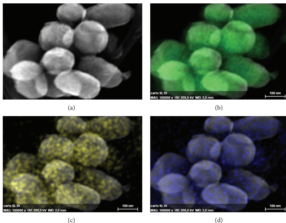
FIGURE 8: Electron microscope images and elemental cartography of m\text{SiO}_2\text{-Eu}(\text{TTA})_3(\text{Phen-Si}) . (a) STEM image, (b) Si cartography, (c) N cartography, and (d) Eu cartography.
