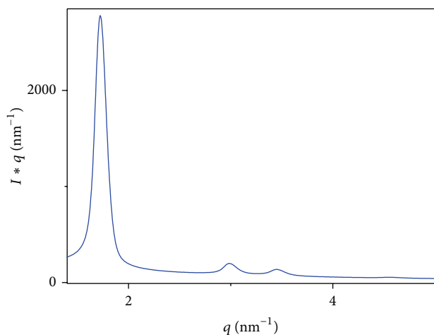
FIGURE 5: SAXS diagram of synthesized mesoporous silica nanoparticles ( mSiO_2 ).
