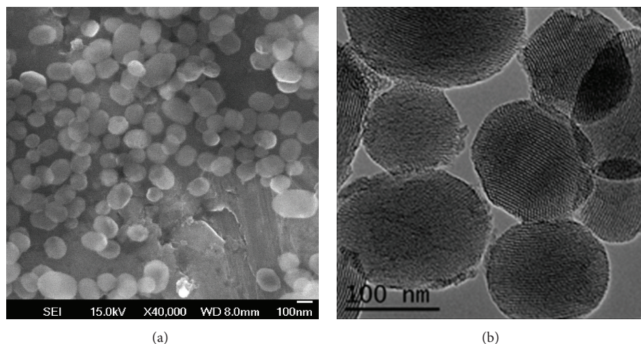
FIGURE 4: SEM (a) and TEM (b) images of synthesized mesoporous silica nanoparticles ( mSiO_2 ).
