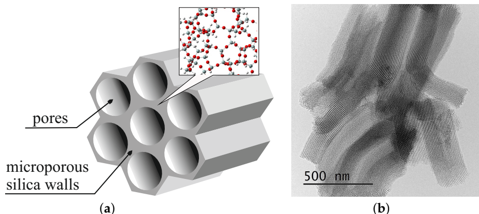
Figure 1. The structure of SBA-15 type mesoporous silica: a scheme (a); and a TEM micrograph (b).
