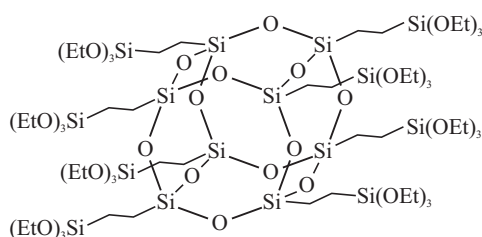
Figure 7. The cage-like structure of octa(triethoxysilyl)ethylpolyhedral oligomeric silsesquioxane. Et, ethyl groups.
