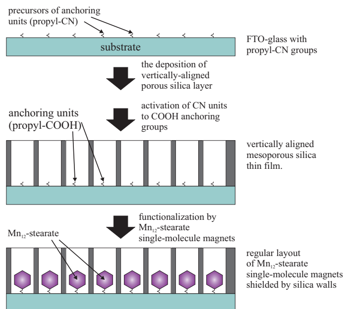
Figure 11. A schematic representation of the synthesis procedure for fabrication of vertically aligned thin mesoporous silica layers containing singular Mn 12 -stearate molecules at the bottom of channels.
