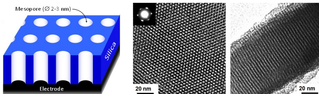
Figure 8. A schematic illustration of a vertically-oriented mesoporous silica film electrogenerated onto an electrode surface and typical corresponding TEM micrographs (top and cross-section views).
