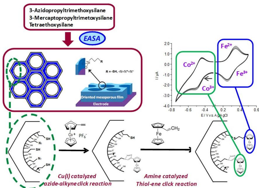
Figure 9. An illustration of the elaboration of oriented azide-thiol-functionalized mesoporous silica film by EASA and subsequent derivatization of azide groups by reaction with an alkyne derivative and the thiol ones with an alkene one.
