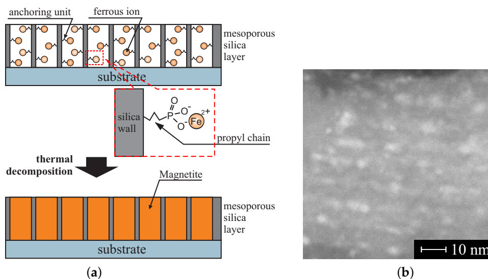
Figure 15. The general illustration the procedure of magnetite synthesis by the use of silica nanoreactors (a); and resulting nanoparticles of magnetite obtained inside SBA-15 (TEM image) (b).
