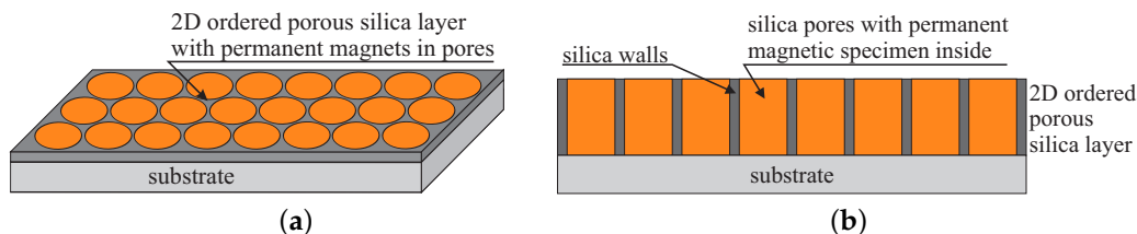
Figure 14. The structure of the silica-based memory storage device: perspective projection (a); and cross section (b).
