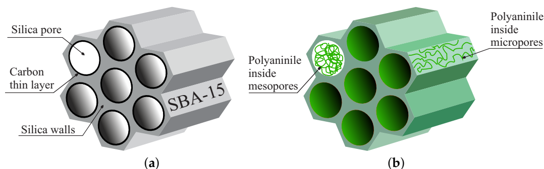
Figure 3. A schematic representation of the porous silica-based composite materials for the application of supercapacitors: (a) a carbon-lined SBA-15 mesoporous silica; and (b) SBA-15 containing polyaniline chains inside its structure.
