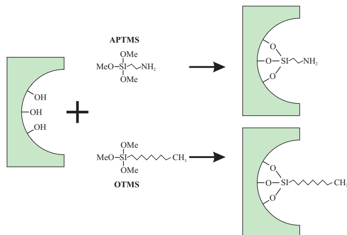
Figure 5. A schematic presentation of the silylation reaction presented in [98] and possible configuration of the SBA-15 after surface modification. Me, methyl groups.
