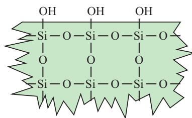
Figure 4. A schematic illustration of the silica structure with surface hydroxyl units. The structure is simplified and presented in a 2D plane.
