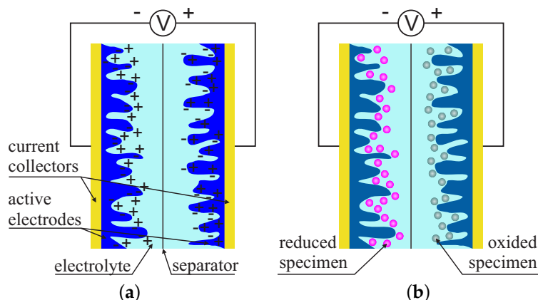
Figure 2. A schematic illustration of supercapacitors: an electrical double-layer capacitor (a); and a pseudocapacitor (b).
