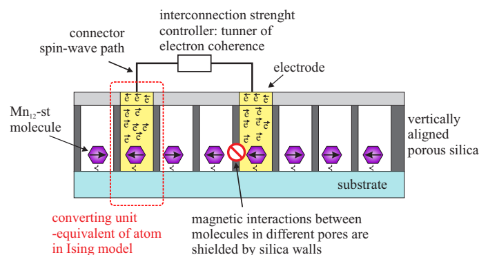
Figure 13. A schematic illustration of the molecular neural network with two interacting molecular neurons (processing units).
