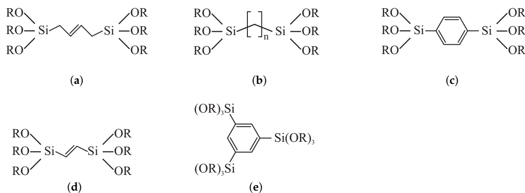
Figure 6. A schematic representation of the bridged silsesquioxane monomers applied in [111] ((a,b) for n = 2, 3, 6, 8, 10 (c)) and in [112] ((b) for n = 1, 2 , (c–e)). R = C_2H_5 .
