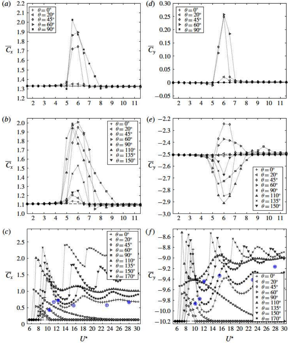
FIGURE 5. (Colour online) Time-averaged (a–c) in-line and (d–f) cross-flow force coefficients as functions of the reduced velocity, over a range of vibration angles, for (a,d) \alpha = 0 , (b,e) \alpha = 1 , (c,f) \alpha = 3 . In each plot, the time-averaged value of the force coefficient in the rigidly mounted cylinder case is indicated by a dashed line. In (c,f), the three-dimensional simulation results are denoted by circled blue symbols.
