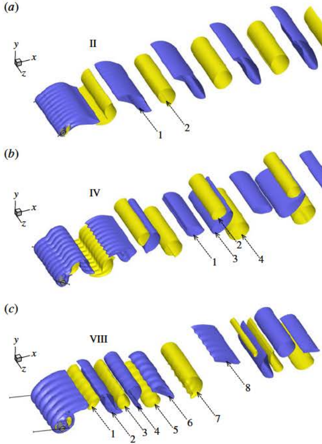
FIGURE 13. (Colour online) Instantaneous iso-surfaces of spanwise vorticity, for \alpha = 3 ( \omega_z = \pm 0.07 ): (a) II pattern, (\theta, U^*) = (20^\circ, 10) ; (b) IV pattern, (\theta, U^*) = (150^\circ, 12) ; (c) VIII pattern, (\theta, U^*) = (170^\circ, 28) . Positive/negative vorticity values are plotted in yellow/blue. Dashed arrows indicate the vortices shed over one oscillation cycle. The trajectory of the cylinder is indicated by a segment. Part of the computational domain is shown.
