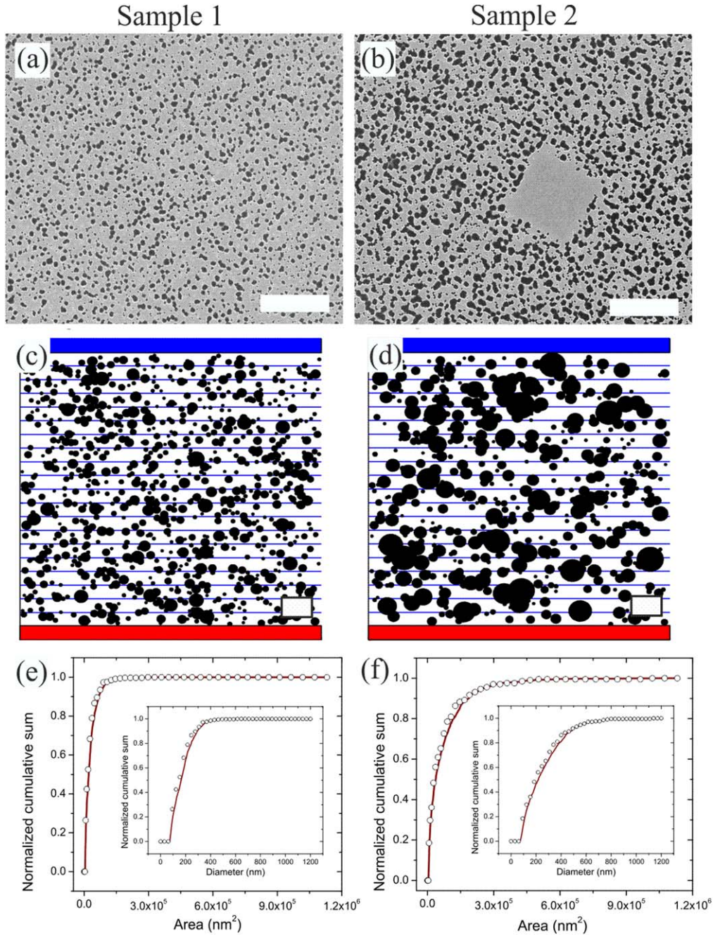
Figure 1. SEM images of (a) Sample 1 with 25% filling fraction and (b) Sample 2 with 37% filling fraction and the detail of the heating island located in the center of the sample. Scale bar 5\ \mu\text{m} . Theoretical samples used for MC simulations corresponding to (c) Sample 1 and (d) Sample 2. Red and blue bars correspond to the hot and cold side of the sample, respectively. Scale bar 1\ \mu\text{m} . Normalized cumulative sum of the areas of the pores in (e) Samples 1, (f) Sample 2; circles correspond the experimentally measured distributions from SEM, red curves are the modeled distributions derived from figures (c) and (d). Insets correspond to the cumulative sum of the diameters, assuming circular pores for a given area distribution.
