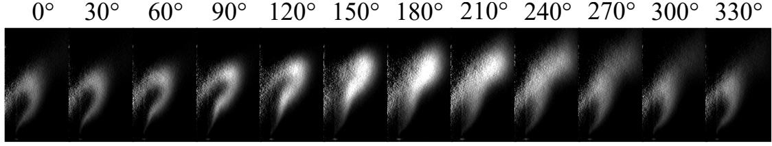
Fig. 6 Phased \text{CH}^* chemiluminescence of the flame during one cycle of oscillation. Images are averaged over 600 cycles.
