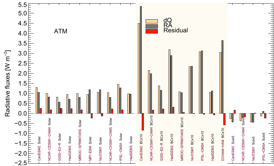
Figure 3. The longwave (LW) fast radiative cooling (dQ), where the LW instantaneous radiative cooling is zero (or extremely small). For all solar cases the LW instantaneous radiative cooling is zero, for BCx10 the LW instantaneous radiative cooling is zero or very small, and for some of the Sulx5 cases the LW instantaneous radiative cooling is zero (for those models neglecting aerosol-cloud interactions). The LW dQ is the output from the PDRMIP models, and the LW rapid adjustment (RA) is calculated by the radiative kernel methods. The residuals are the difference between LW dQ and the LW RA.
