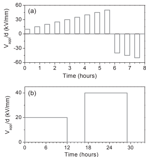
Fig. 2: Short (a) and long (b) term protocols for space charge measurements
