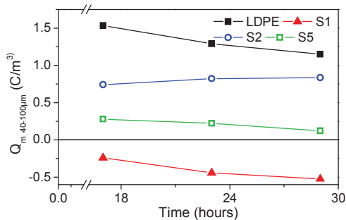
Fig. 5: Charge density averaged from 40 \mu\text{m} to 100 \mu\text{m} from the cathode during the 40 kV/mm step along the long term protocol
