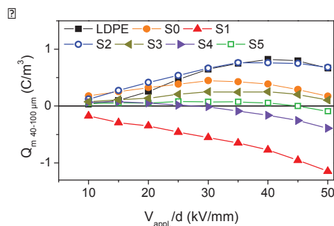
Fig. 4: Charge density averaged from 40 \mu\text{m} to 100 \mu\text{m} from the cathode at the end of each voltage step for the different tested samples
