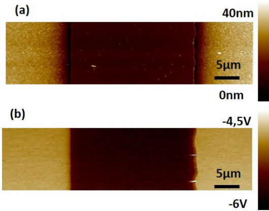
Fig. 2. (a) Topography and (b) surface potential map over Al/SiN x sample in FM-KPFM mode. Electrodes in cross-section.
