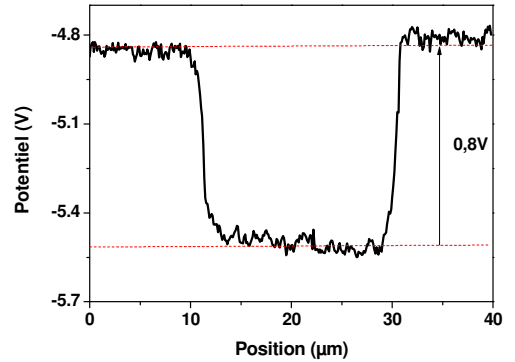
Fig. 3. Surface potential profile between electrodes measured on Al/SiN x sample by FM-KPFM
