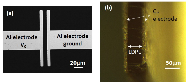
Fig. 1. Optical microscope pictures of (a) Al electrodes embedded in \text{SiN}_x thin layer and (b) LDPE layer between Cu-electrodes in cross-section.
