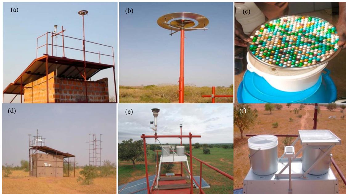
Figure 2. (a and b) Total deposition passive collector at Cinzana station (Mali) and (c) view of the collecting frisbee full of marbles and (d–f) MTX collector at Banizoumbou station (Niger).
