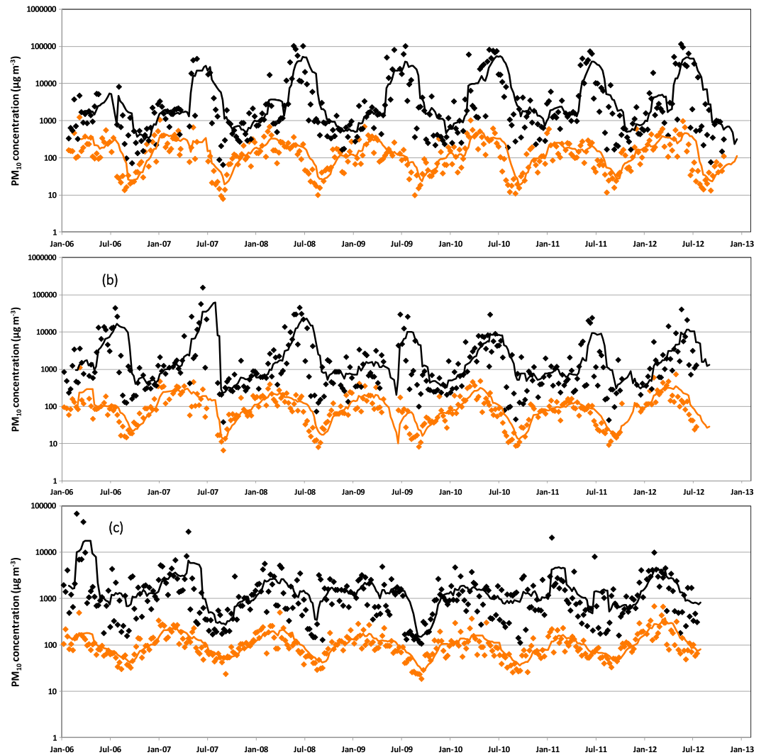
Figure 7. Mean (orange) and maximum (black) PM 10 concentration over the sampling duration of the total depositions fluxes from January 2006 to December 2012 in (a) Banizoumbou (Niger), (b) Cinzana (Mali), and (c) M'Bour (Senegal). The lines correspond to a sliding averaged performed over eight successive data, i.e., about 8 weeks.
