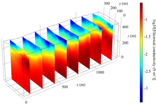
Fig. 16. 3D electrical conductivity tomogram (in \text{S} \cdot \text{m}^{-1} ) of the Krafla Site 1 in Iceland. The inverted model of electrical conductivity reveals the presence of a low electrical conductivity near surface layer, which is identified as unaltered porous basalt. In turn, this layer covers a high conductivity cap corresponding to the smectite-zeolite cap of the geothermal system.
