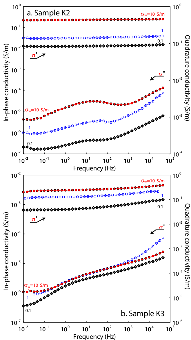
Fig. 6. Spectral induced polarization data (in-phase conductivity \sigma' and quadrature conductivity \sigma'' ) for two volcanic samples from Iceland volcano Krafla in the frequency range 10 mHz–45 kHz. a. In-phase and quadrature conductivities spectra of core sample K2. b. In-phase and quadrature conductivities spectra K3. The induced polarization measurements are performed at three pore-water conductivities (0.1, 1 and 10 S m -1 , NaCl, 25 °C).
