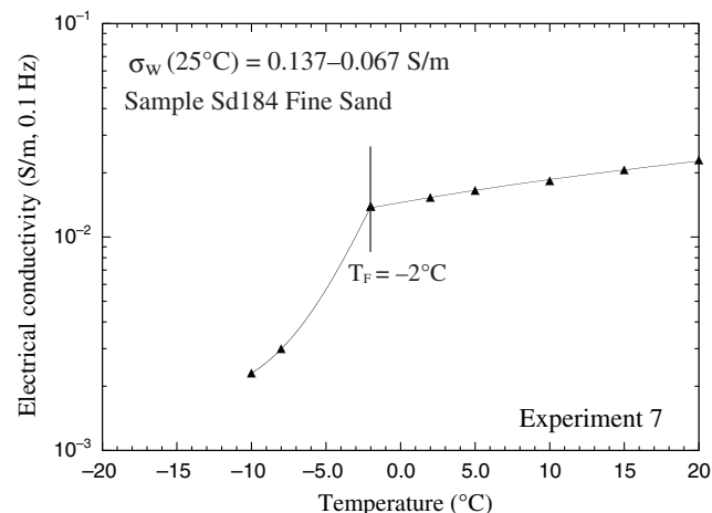
Figure 2. Evolution of the electrical conductivity as a function of the temperature T ( ^{\circ}\text{C} ) for the background material (experiment 7). Below the freezing temperature, the fit is done with the exponential freezing curve as described earlier. Above the freezing temperature, the data are fitted by the linear relationship corresponding to equation 13. The change of slope through the freezing point is due to the formation of ice in the pore space of the material. The highest value of pore water conductivity corresponds to the value of the pore water used to saturate the sand. The lowest value corresponds to the value measured after 240 h of experiments including several cycles of freezing and thawing.
