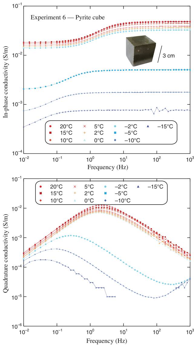
Figure 8. Results of experiment 6 with a pyrite cube immersed in water-saturated sand.
