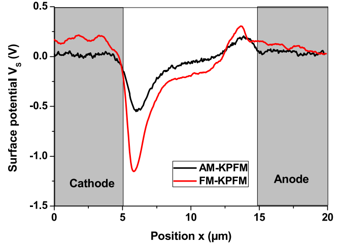
Figure 2. Comparison of surface potential profiles measured by the AM-KPFM and FM-KPFM techniques for an inter-electrode distance of 10 \mu\text{m} after 1 h of polarization ( -40 \text{ V} applied to the left electrode and ground applied to the right one during polarization).
