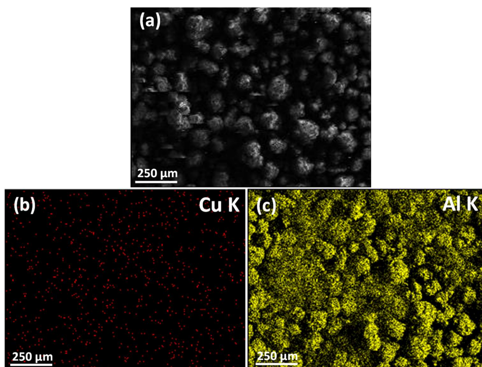
Figure 6. Example of SEM image (a) and EDX analyses for 1 wt.% Cu/Al 2 O 3 catalyst (b and c)
