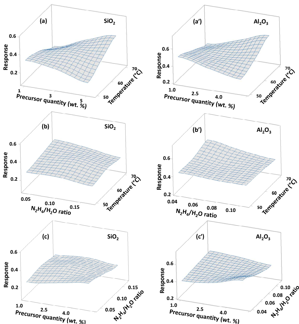
Figure 4. 3D surface plots depicting the relationship between response and two different predictor variables; Response vs (a) temperature & precursor quantity (b) temperature & \text{N}_2\text{H}_4/\text{H}_2\text{O} , (c) \text{N}_2\text{H}_4/\text{H}_2\text{O} & precursor quantity for \text{SiO}_2 . Response vs (a') temperature & precursor quantity (b') temperature & \text{N}_2\text{H}_4/\text{H}_2\text{O} , (c') \text{N}_2\text{H}_4/\text{H}_2\text{O} & precursor quantity for \text{Al}_2\text{O}_3 .
