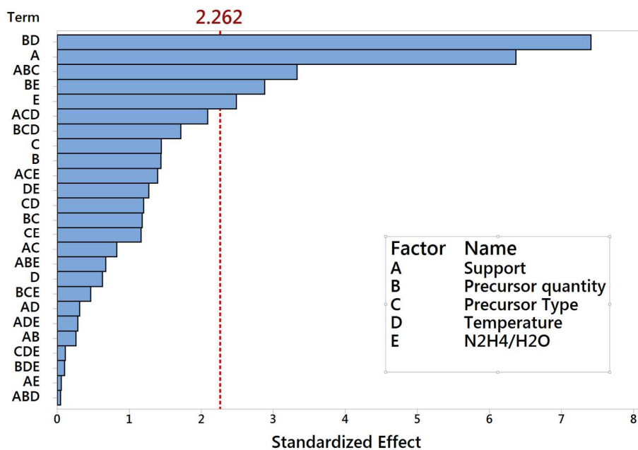
Figure 2. Pareto chart of the standardized effect of factors and their interactions in DoE experiments
