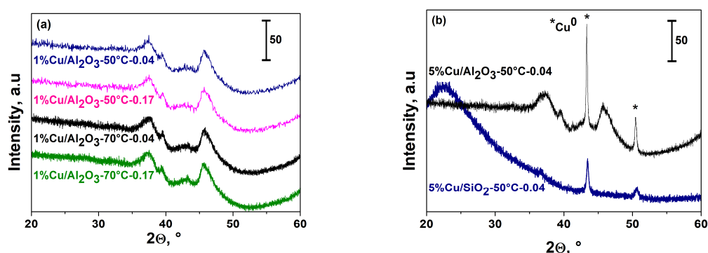
Figure 5. XRD patterns when (a) 1 wt.% of Cu precursor were used during syntheses under different conditions and (b) 5 wt.% of Cu precursor were used during syntheses at 50 °C and N 2 H 4 /H 2 O molar ratio of 0.04
