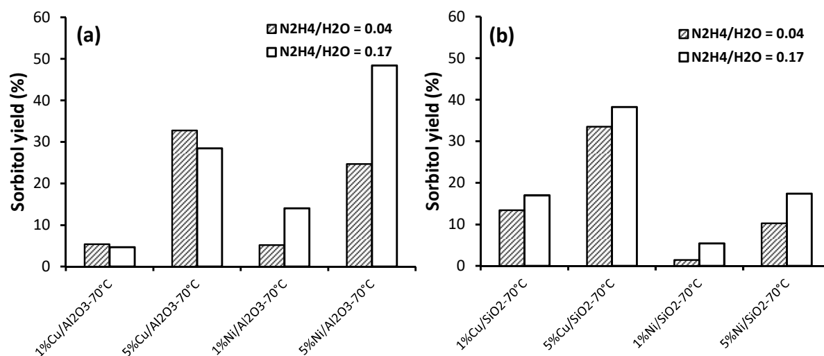
Figure 10. Sorbitol yields with (a) Alumina-supported and (b) Silica-supported catalysts synthesized at two different hydrazine/water ratio at 70 °C (Test conditions: Catalyst amount=10 mg, 3 mL of glucose solution (1wt.%), T=130 °C, P H 2 = 30 bar, t = 4h)
