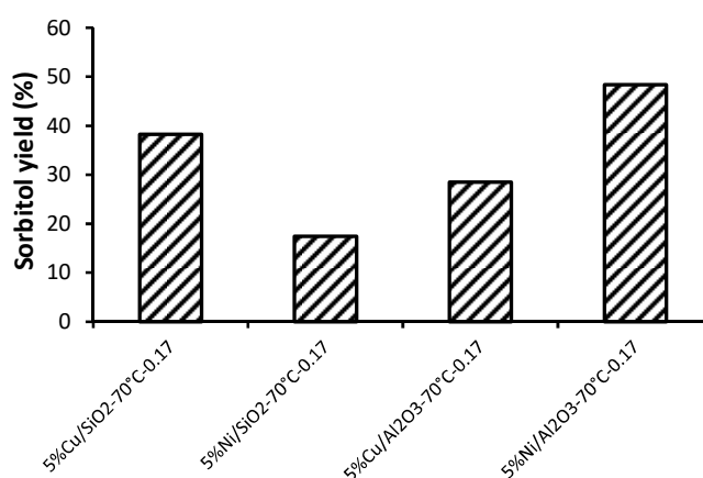
Figure 11. Sorbitol yield on 5 wt.% metal loaded catalysts synthesized at 70 °C and hydrazine/water molar ratio = 0.17. (Test conditions: Catalyst amount=10 mg, 3 mL of glucose solution (1wt.%), T=130 °C, P H 2 = 30 bar, t = 4h)
