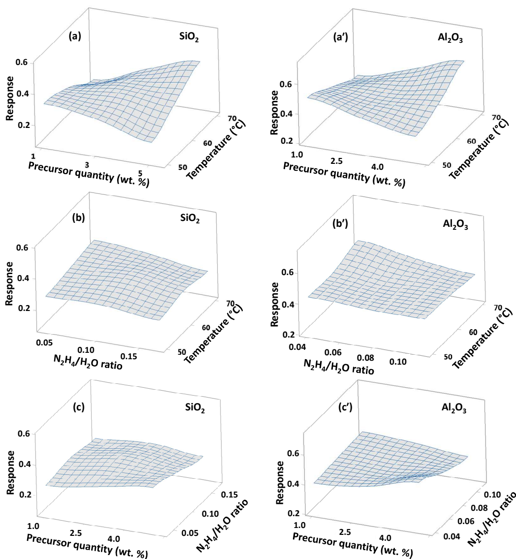
Figure 4. 3D surface plots depicting the relationship between response and two different predictor variables; Response vs (a) temperature & precursor quantity (b) temperature & N_2H_4/H_2O , (c) N_2H_4/H_2O & precursor quantity for SiO_2 . Response vs (a') temperature & precursor quantity (b') temperature & N_2H_4/H_2O , (c') N_2H_4/H_2O & precursor quantity for Al_2O_3 .
