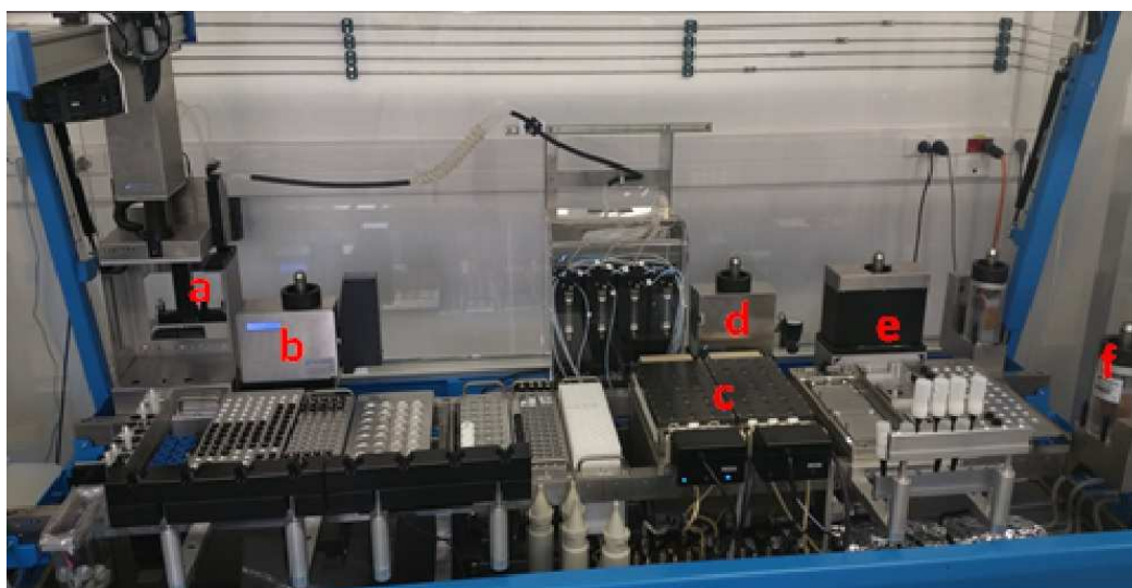
Figure 1. The Chemspeed Catimreg workstation used for catalysts preparation comprising (a) 4 Needles-Head (4 NH), (b) Gravimetric Dispensing Unit for Viscous solution (GDU-V), (c) Isynth reactor blocks, (d) Solid Dispensing Unit (SDU), (e) Screw capper and (f) Multigripper
