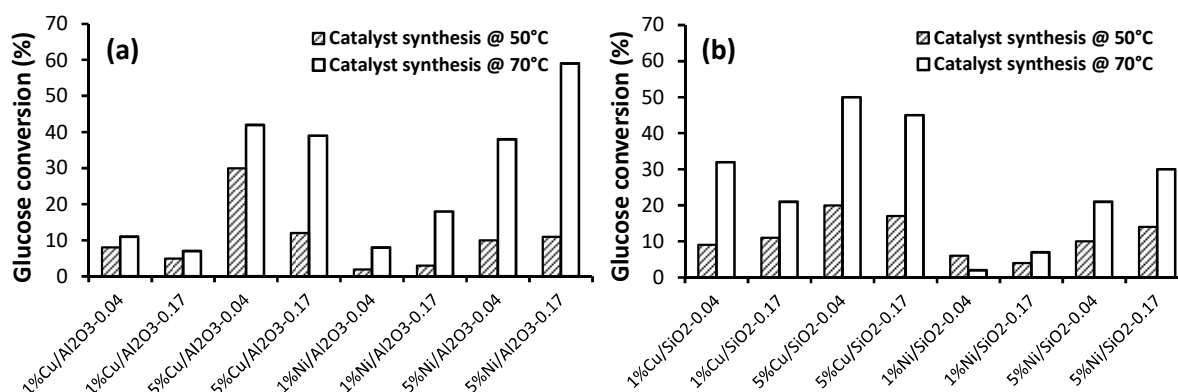
Figure 8. Glucose conversions with (a) Alumina-supported and (b) Silica-supported catalysts synthesized at temperatures 50 and 70 °C. (Test conditions: Catalyst amount=10 mg, 3 mL of glucose solution (1 wt.%), T=130 °C, P_{H_2} = 30 bar, t = 4h)
