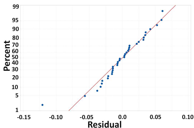
Figure 3. Normal probability plot of residuals in the model (Response = Obtained/Expected)
