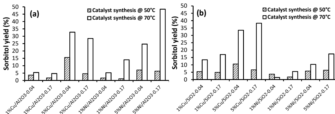
Figure 9. Sorbitol yields with (a) Alumina-supported and (b) Silica-supported catalysts synthesized at temperatures 50 and 70 °C. (Test conditions: Catalyst amount=10 mg, 3 mL of glucose solution (1 wt.%), T=130 °C, P_{H_2} = 30 bar, t = 4h)
