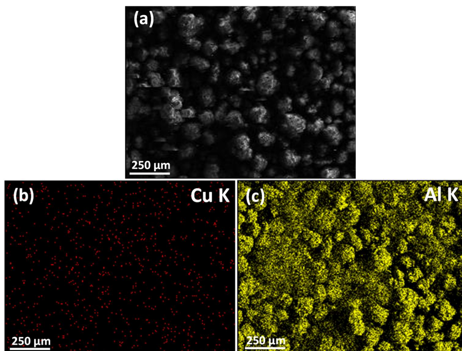
Figure 6. Example of SEM image (a) and EDX analyses for 1 wt.% Cu/Al 2 O 3 catalyst (b and c)
