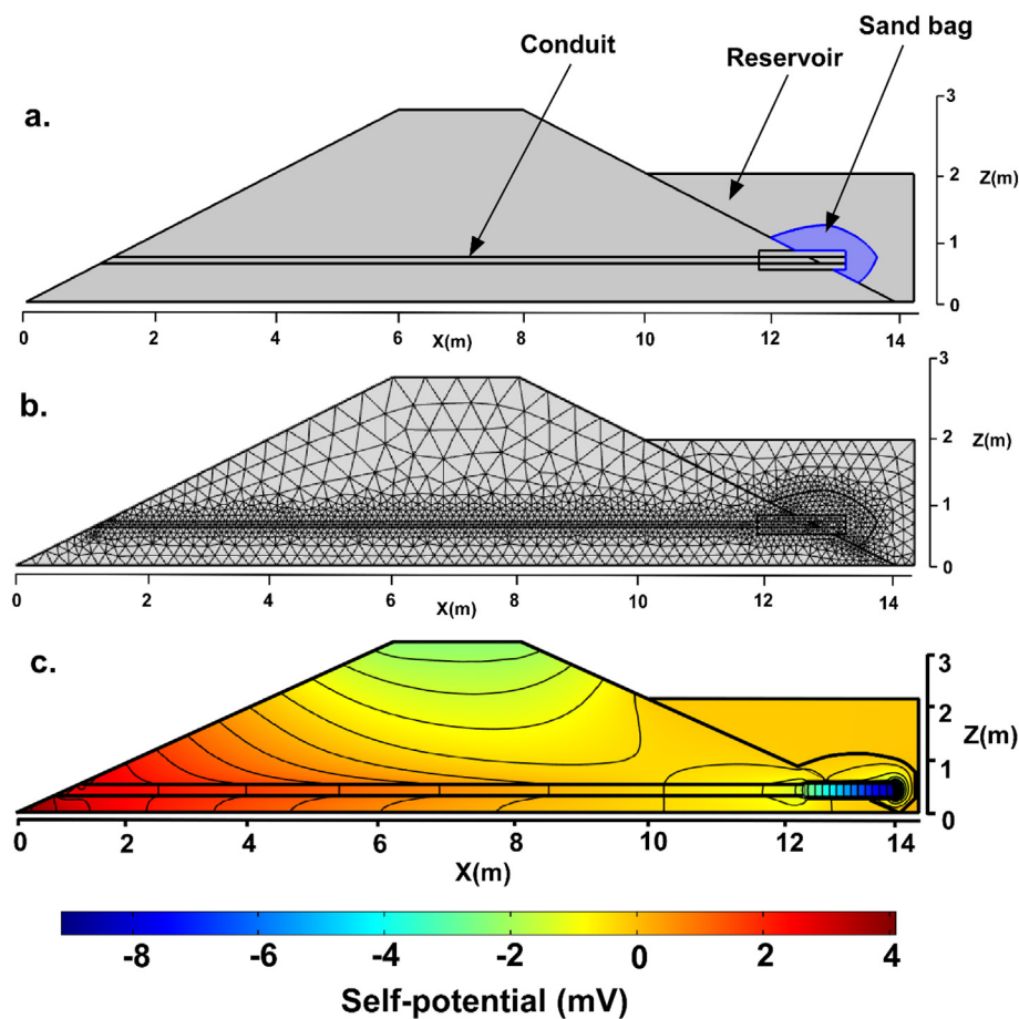
Fig. 11. Numerical modelling of modification of the dam. a. Vertical view of the dam. b. Finite element mesh. c. Self-potential distribution after adding a porous material is added at the entrance of the conduit. The blue domain models the porous material added to the entrance of the conduit. This figure shows how the modification of the dam was modeled. The porous material placed at the entrance of the area of infiltration was modeled as a new subdomain (blue domain) which is meshed and identified through each hydraulic and electric conductivities. The self-potential anomaly is relatively strong (approximately -9\text{ mV} with respect to the crest) but very localized in the vicinity of the inflow area. (For interpretation of the references to colour in this figure legend, the reader is referred to the web version of this article.)
