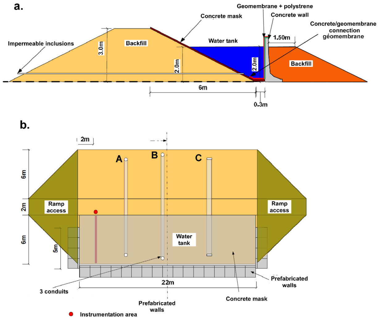
Fig. 1. Sketch of the geometry of the dam. a. Vertical view of the dam. b. View from above the dam. The dam is connected to a water tank that is made by assembling some prefabricated walls. Three high permeability conduits (denoted A, B and C on the figure) are inserted across the core of the dam. This allows for creating preferential flow paths for the water contained in the water reservoir. A concrete mask is put on the downstream part of the core to make it impermeable.
