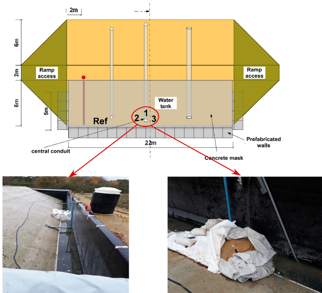
Fig. 12. Representation of the proposed modification of the dam. Three electrodes numbered 1, 2 and 3 are located on the top of the sand. The reference electrode is placed in the tank and is denoted by Ref on the figure. The lower left image shows a side view of the tank while the lower right image shows a view of the sand bag and the electrodes.
