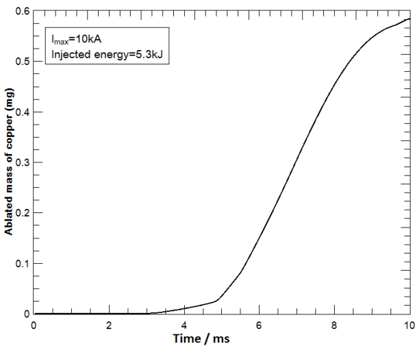
Figure 5. Ablation of copper material with time t .
