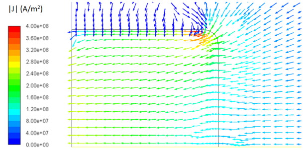
Figure 3. Current density vector close to the electrode for time t=5ms .
