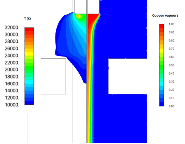
Figure 2. Temperature and copper mass fraction for time t=5ms .
