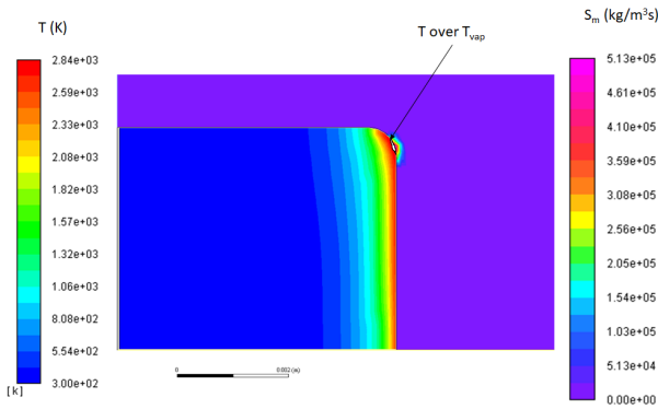
Figure 4. Temperature in the electrode (left) and mass source term due to copper ablation (equation (7)) at t=5ms .
