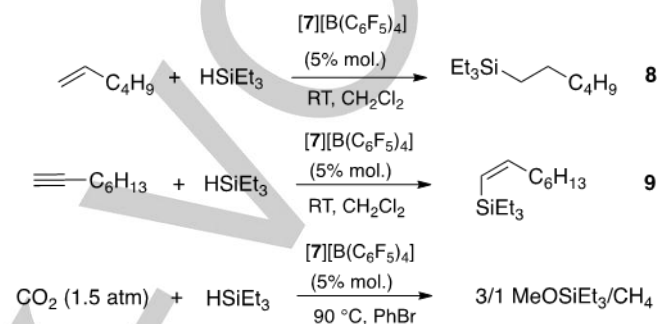
Scheme 4. Hydrosilylation reactions catalyzed by [7][\text{B}(\text{C}_6\text{F}_5)_4] .
