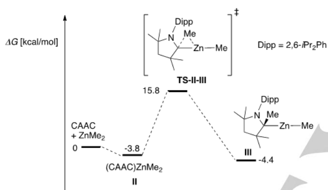
Figure 2. DFT-computed (B3LYP/6-31+G**, toluene) reaction profile for the formation of model III from CAAC and \text{ZnMe}_2 .
