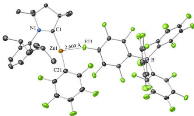
Figure 5. Molecular structure of ion pair [(CAAC)Zn–C 6 F 5 ][B(C 6 F 5 ) 4 ] ( [7][B(C 6 F 5 ) 4 ] , ORTEP plot with thermal ellipsoids shown at the 30% probability level). Hydrogen atoms are omitted and selected atoms are labelled for clarity.
