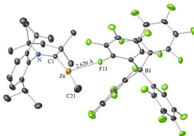
Figure 3. Molecular structure of [(\text{CAAC})\text{Zn–Me}][\text{B}(\text{C}_6\text{F}_5)_4] ( [\text{5}][\text{B}(\text{C}_6\text{F}_5)_4] ), ORTEP plot with thermal ellipsoids shown at the 30% probability level). Hydrogen atoms are omitted and selected atoms are labelled for clarity. Selected distances (Å) and angles ( ^\circ ): Zn–C(1) = 1.976(3), Zn–C(21) = 1.913(4), Zn⋯F(11) = 2.620(3), C(1)–Zn–C(21) = 170.2(2).
