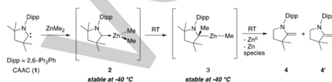
Scheme 1. Reactivity of carbene CAAC 1 with ZnMe 2 .
