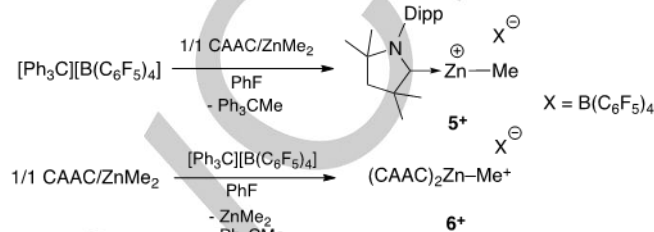
Scheme 2. Synthesis of CAAC-supported Zn organocations 5 + and 6 + as \text{B}(\text{C}_6\text{F}_5)_4^- salts.
