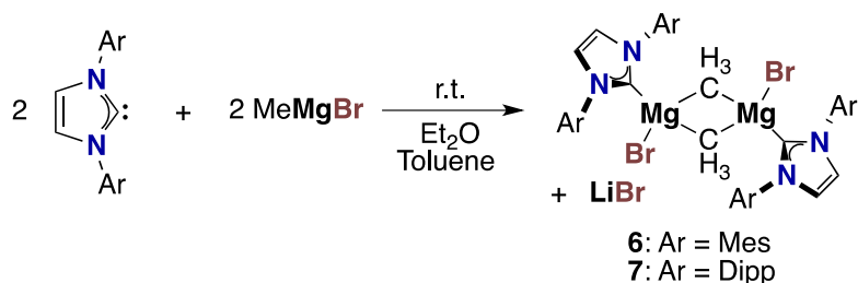
Scheme 3. Synthesis of species 6 and 7
