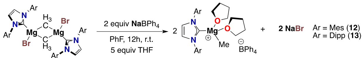
Scheme 5. Synthesis of NHC–Mg(II) alkyl cations 12-13
