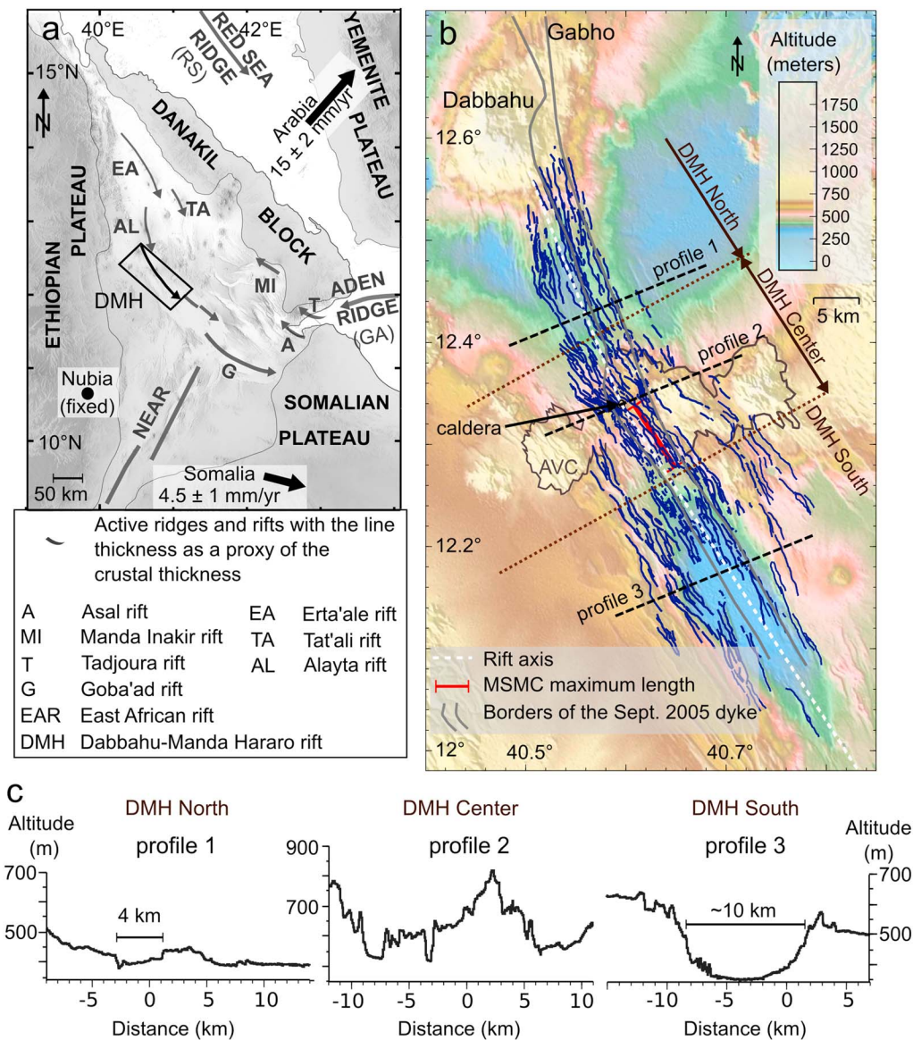
Figure 2. magmato-tectonic setting of Dabbahu-Manda-Hararo (DMH) rift. (a) magmato-tectonic rifts composing the three branches of the Afar triple junction, the Red Sea and Aden ridges as well as the system of the east African rifts. The arrows associated to rift segments represent the direction of rift propagation. After Figure 26 from Manighetti, Tapponnier, et al. (2001). (b) Topographic map of DMH rift including the mapping of the 668 faults considered in this study (blue lines). In addition to the mid-segment magma chamber, other magma sources are also indicated: Ado'Ale volcanic complex, Dabbahu and Gabho volcanoes. Along the rift axis, three rift segments are defined (north, center, and south, dark brown dotted lines) based on morphological and structural observations (see text for more details). Topographic profiles (black dashed lines) across these three segments are shown in (c).
