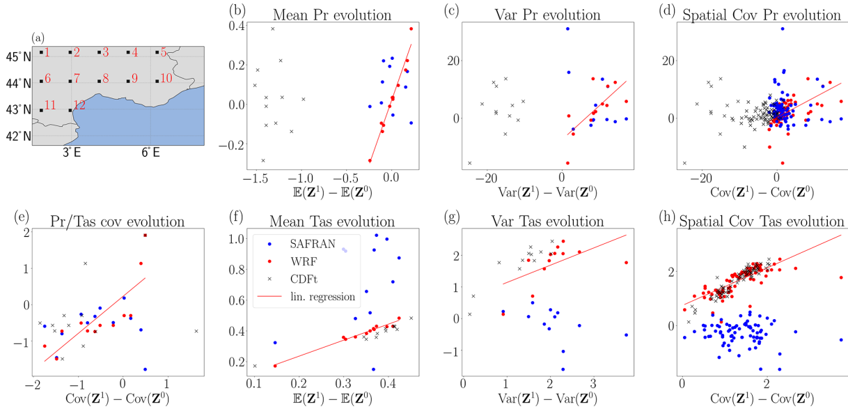
Figure 5. (a) Map of the southeast of France. The 12 black squares are the locations where corrections are performed. (b–h) The x axis of the panels is the evolution of the correction with dOTC. The y axis of panels (b)–(h) is the evolution of WRF in red and the evolution of SAFRAN in blue. The red line is the linear regression between the evolution of correction and the evolution of WRF. The black cross markers are the scatterplots between the evolution of correction with CDFt and evolution of WRF. (b) Evolution of mean precipitation, i.e., difference between the projection period and the calibration period. (c) Evolution of variance of precipitation. (d) Evolution of spatial covariance of precipitation. (e) Evolution of covariance between precipitation and temperatures. (f) Evolution of mean temperatures. (g) Evolution of variance of temperatures. (h) Evolution of spatial covariance of temperatures.
