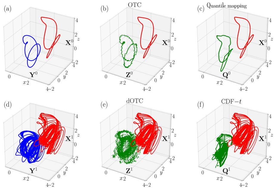
Figure 4. Random variables generated by the Lorenz (1984) model, OTC, dOTC, quantile mapping and CDF- t . (a) Biased random variable \mathbf{X}^0 (red) and references \mathbf{Y}^0 (blue) for time period 0. (b) Biased random variable \mathbf{X}^0 (red) and correction \mathbf{Z}^0 with OTC (green). (c) Biased random variable \mathbf{X}^0 (red) and correction \mathbf{Q}^0 with quantile mapping (green). (d) Biased random variable \mathbf{X}^1 (red) and references \mathbf{Y}^1 (blue) for time period 1. (e) Biased random variable \mathbf{X}^1 (red) and correction \mathbf{Z}^1 with dOTC (green). (f) Biased random variable \mathbf{X}^1 (red) and correction \mathbf{Q}^1 with CDF- t (green).
