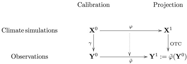
Figure 2. Estimation of the unobserved random variable \mathbf{Y}^1 . The random variables \mathbf{X}^0 , \mathbf{X}^1 and \mathbf{Y}^0 are known. Plans \gamma and \varphi are the optimal joint laws in the sense of Eqs. (2)–(4). \tilde{\varphi} is the evolution of \mathbf{Y}^0 estimated from \gamma and \varphi . OTC is used to correct \mathbf{X}^1 with respect to the estimation of \mathbf{Y}^1 .
