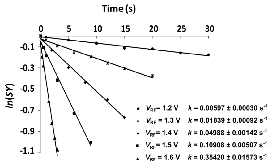
Figure 4- Kinetic plots of H-G ref at different resonant activation amplitudes.
