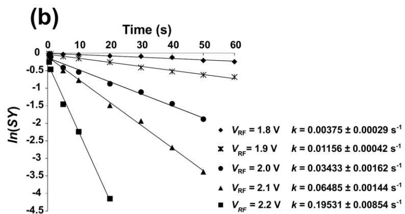
Figure 5- (a) MS/MS spectrum of the m/z 1252 [(\text{Zn(II)}@1+3)\text{-H}]^+ precursor obtained using low-energy CID at 1.9 V excitation voltage and 50 s decomposition time. Due to the employed resonant excitation, only the monoisotopic peak of the precursor ion ( m/z 1252) is decomposed. (b) Kinetic plots of [(\text{Zn(II)}@1+3)\text{-H}]^+ obtained at different excitation amplitudes.
