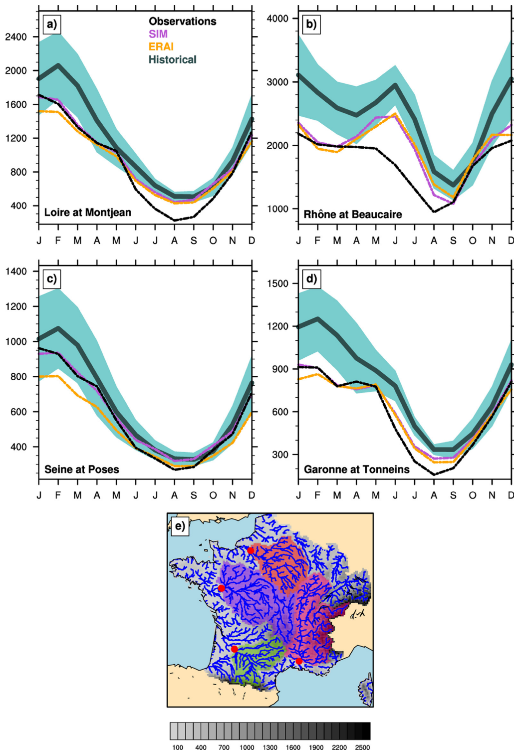
Fig. 1. (a–d) Climatological annual cycle of streamflows ( \text{m}^3 \text{s}^{-1} ) on the 1979–2005 period in the observations (black), the Safran–Isba–Modcou analysis (purple), as simulated by Isba–Modcou driven by the downscaling of the ERA-Interim reanalysis (yellow) and simulated by Isba–Modcou driven by the downscaling of the CMIP5 GCMs on the historical period (cyan). The shading represents the uncertainties range due to GCMs. It is estimated by a 1.64 standard deviation between the simulations, weighted by the number of members for each GCM. (e) Hydrographic network of the Modcou model and river basin of the four main French river in color: the Seine at Poses (red), the Loire at Montjean-sur-Loire (blue), the Rhône at Beaucaire (pink) and the Garonne at Tonneins (green). The stations where the streamflows are studied are marked by a red dot.
