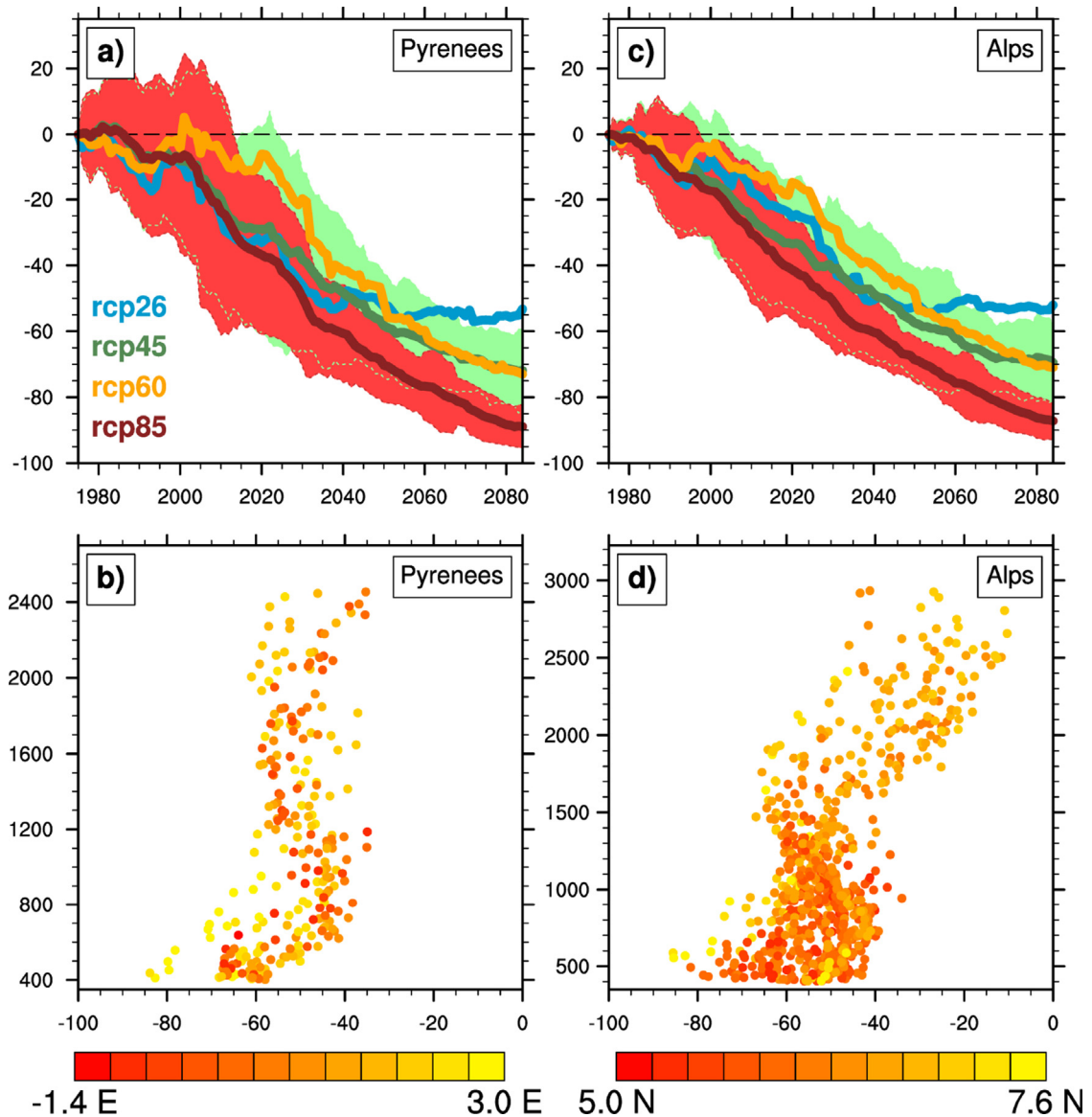
Fig. 6. Top: ensemble mean of the averaged annual snow mass evolution (%) relative to the 1960–1990 period for the RCP2.6 (blue), the RCP4.5 (green), the RCP6.0 (yellow), and the RCP8.5 (red) scenario on the Pyrenees mountains (a) and the French Alps mountains (c). The colored shadings represent the estimation at [5–95%] of the uncertainty range due to GCMs for the RCP4.5 and RCP8.5 scenario, estimated by a 1.64 standard deviation between simulations. Data have filtered with a 31-year running mean. Bottom: relative changes of the daily annual maximum of the snowpack (%) for the RCP4.5 scenario in each grid cell according to their respective altitude (m) on the French Pyrenees mountains (b) and the French Alps (d). The each dots are colored according to their longitude (latitude) in the Pyrenees (French Alps).
