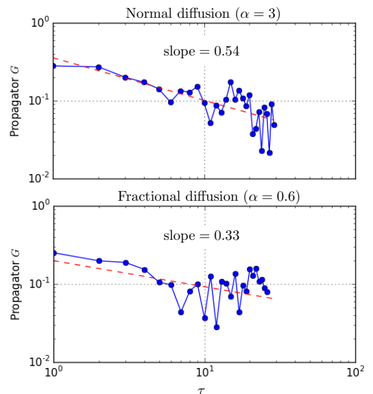
Fig. 2. Fit of the inverted propagator G_\tau for a random order flux simulation: (top) in the normal diffusion case ( \alpha = 3 > 1 ) with slope 0.54 \approx 1/2 , and (bottom) in the fractional diffusion case ( \alpha = 0.6 < 1 ) with slope 0.33 \approx \alpha/2 .
