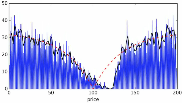
Fig. 1. Numerical simulation of the latent order book during a constant rate buy meta-order execution. The red dashed line corresponds to the equilibrium order book from which the simulation started at t = 0 .
