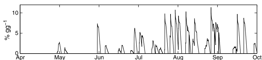
Figure 1. Gravimetric soil moisture at 1 cm estimated from measurements performed at 5 cm depth, Agoufou site, 2008.
