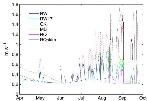
Figure 5. Friction threshold velocities depending on the soil moisture and according to various drag partition schemes (RW: Raupach–Walter, RW17: RW with the \sigma parameter computed from the Agoufou obstacles’ dimensions, OK: Okin (integrated value), MB: Marticorena and Bergametti, RQ: Raupach–QUIC, and RQskim: RQ with a skimming flow value), Agoufou site, 2008.
