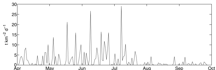
Figure 7. Simulated dust emission from the surface without vegetation, taking into account soil moisture (Bare and Wet case), Agoufou site, 2008.
