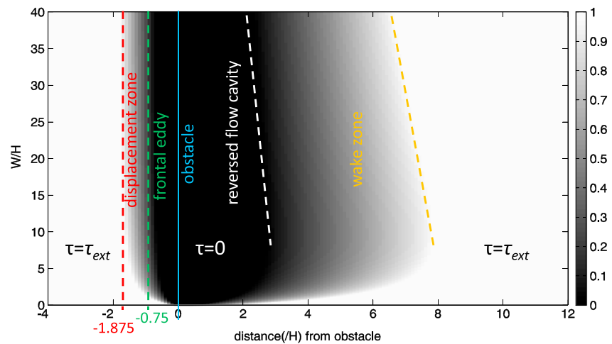
Figure B2. Shear stress ratio \tau/\tau_{ext} varying with d/H (distance to the obstacle divided by the obstacle height) and the aspect ratio W/H (length of the obstacle divided by its height; here W=L ).
