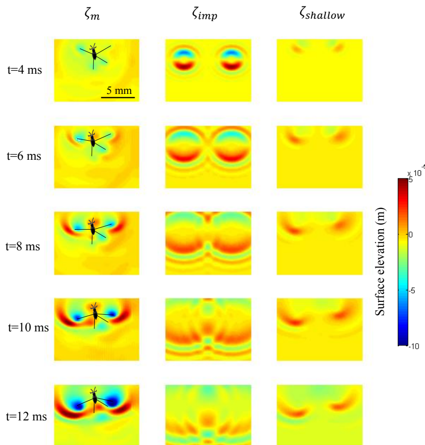
FIGURE 3. Comparison of the experimentally measured surface elevation with theoretical predictions. The 1 st column represents the experimental surface elevation generated during the propulsion of a Gerris paludum individual ( m_{\text{gerris}} = 0.348 mg, V_{\text{gerris}} = 0.38 m.s -1 ). The 2 nd column represents the theoretical surface elevation produced by a single impulse in the direction of motion, with \zeta_{\text{imp}} as expressed in equation (2.13) (Bühler (2007)). The 3 rd column shows the results for continuous forcing in shallow water along the trajectory of the water strider legs (see Eqs. (3.1) and (3.2)).
