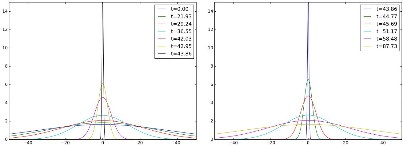
Figure 4: Plot of the breather for \lambda = 0.5 with initial data \exp\left(\frac{1}{2} - \delta x^2\right) with \delta^{-1} = 2 \times 35^2 for some times between 0 and 43.86 (left) and between 43.86 and 87.73 (right).
