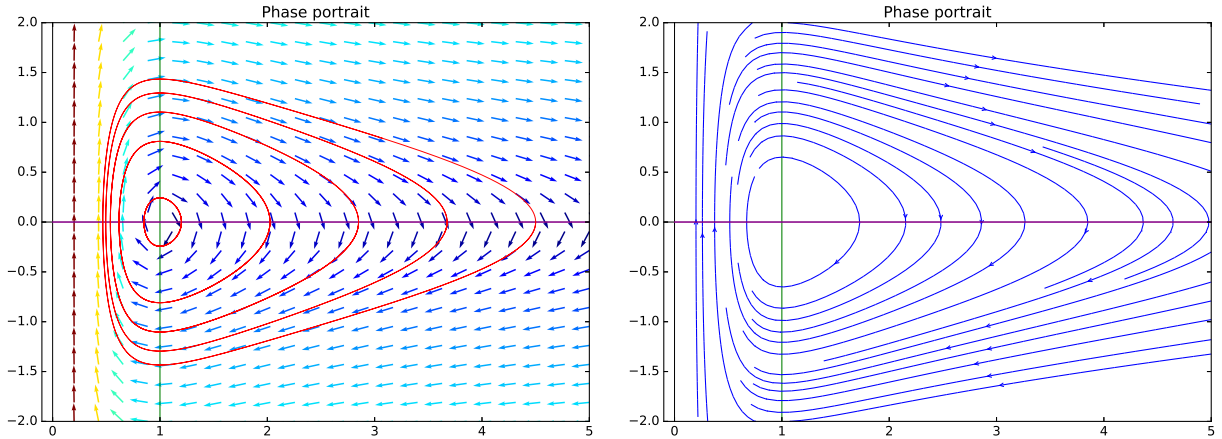
Figure 1: Phase portraits. At the left-hand side, the arrows give the direction of the flow; the green and magenta lines are the horizontal and vertical isoclines respectively; the red lines are some trajectories, which fits the level set of H(p, q) . At the right-hand side, a part of some trajectories are drawn along with the isoclines again.
