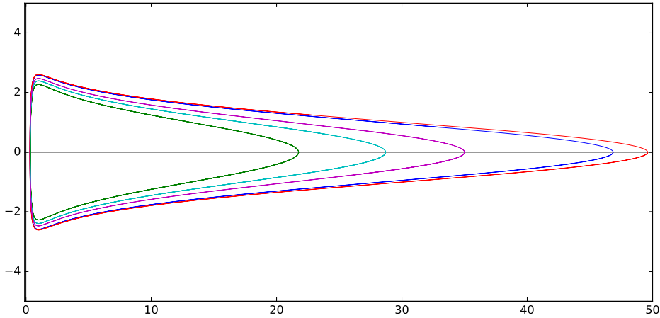
Figure 3: Plot of some trajectories of \tau_\gamma in the phase space for 5 real \gamma between 10 and 50.
