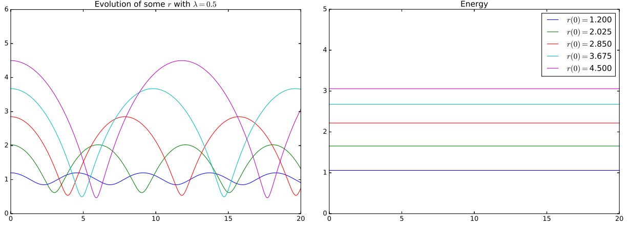
Figure 2: Plot of \tau_\gamma (left) for 5 real \gamma between 1.2 and 4.5 and their energies (right).
