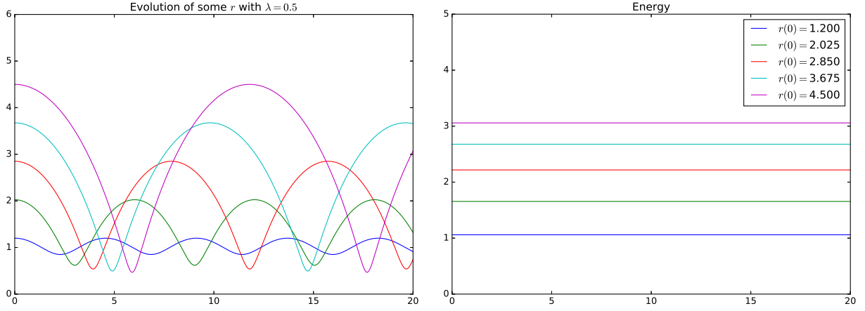
Figure 2: Plot of \tau_\gamma (left) for 5 real \gamma between 1.2 and 4.5 and their energies (right).
