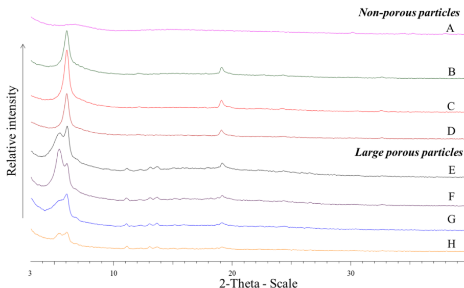
Figure S1: Zoom on the diffractograms of the spray dried samples (A), non-porous particles (B: MX/LEU, C: MX/LEU/HA 0.3 , D: MX/LEU/HA 0.15 ) and LPPs (E: MX/LEU/HA 0.3 /AB 1.5 , F: MX/LEU/HA 0.15 /AB 2 , G: MX/LEU/HA 0.15 /AB 1.5 , H: MX/LEU/HA 0.3 /AB 2 ).
