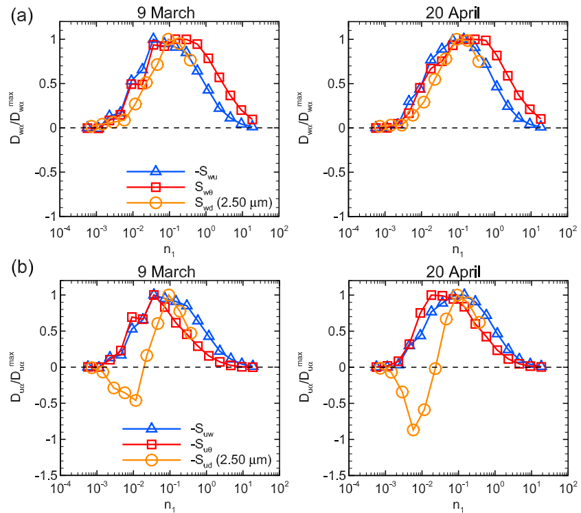
Figure 10. Same as Figure 9 but for the multiresolution decomposition cospectra. On the abscissa, the inverse time scale is normalized by the measurement height z and the mean wind speed at the same height \langle u \rangle such as n_1 = z / (\text{timescale} \times \langle u \rangle) . Equivalent figures for the 7 and 8 March and 14 and 16 April events are available in Figure S6.
