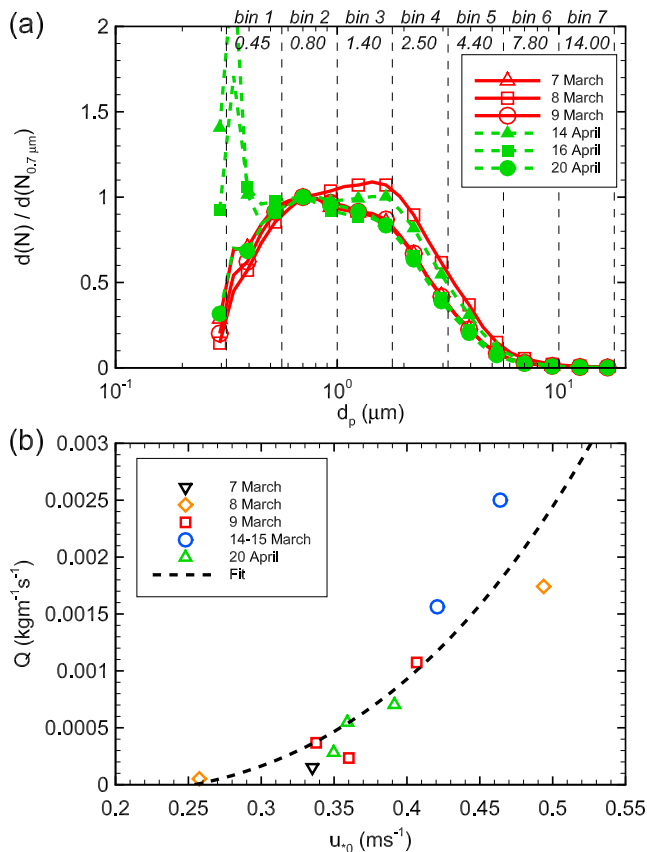
Figure 3. (a) Ensemble-averaged size-resolved dust concentration in number measured by the spectrometer at 3-m height during the six erosion events and normalized by the 0.7- \mu m dust concentration. The seven bins considered in our analysis are indicated with their mean particle size. (b) Saltation flux Q against the surface friction velocity ( u_{*0} ) obtained for the 7–9 March, 14 and 15 March, and 20 April events. The fitted curve in (b) corresponds to the parameterization of Lettau and Lettau (1978) with c = 0.7 (see Dupont et al., 2018). The saltation flux was not measured during the 14 and 16 April events. The 14 and 15 March event was not considered in this study (see section 2.4).
