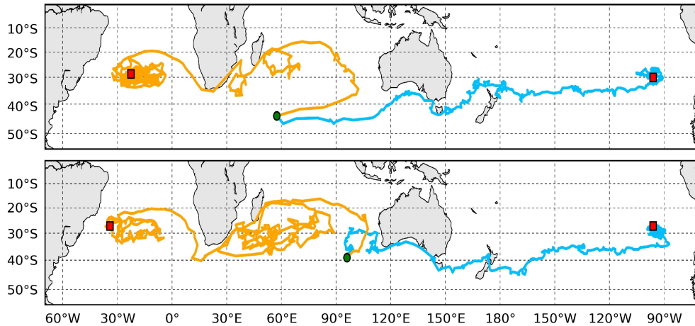
Figure 4: Typical examples of particle trajectories with C-GLORS + surface Stokes drift velocities in orange, and with C-GLORS surface currents only in light blue. The green circles indicate the initial locations and the red squares the final locations after 29 years of advection. The particles were chosen from the 31% (23%) of particles initially located in the South Indian Basin and ending in the South Atlantic Basin (South Pacific) with (without) Stokes drift.
