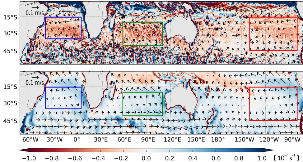
Figure 1: Annual-mean C-GLORS surface currents (top panel) and IOWAGA surface Stokes drift (bottom panel), represented by arrows, and their divergence (shown by the color scale, convergence in red, divergence in blue). The average was made for the year 2014. The colored boxes are the boundaries of the areas used to compute the mean divergence in the main accumulation zones, as discussed in the text.
