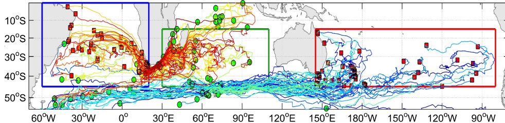
Figure 5: Trajectories of undrogued drifters from the GDP database for drifters that have crossed the South Indian Basin as defined by the green box and that end in the South Atlantic (blue box) or South Pacific (red box). The green circle markers indicate the initial locations, and the red square markers the final locations. The jet colorscale is used to distinguish the trajectories of drifters: The warm (cold) side of the colorscale is used for drifters ending in the South Atlantic (South Pacific).
