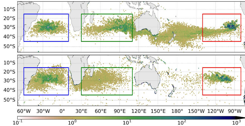
Figure 2: Lagrangian advection of particles by C-GLORS surface current velocities (top panel) and by the IOWAGA Stokes drift added to C-GLORS surface current velocities (bottom panel). These maps show the particle concentration after 29 years of a simulation that cycled 5 times over the 2010-2016 period for input velocities. The color scale is the concentration of particles per grid cell with a log scale. The colored boxes are boundaries used to display the time evolution of the particles and to compute the percentage of particles from the South Indian Basin ending in the South Atlantic or the South Pacific Basin. The black dots represent the center of mass of the concentration of particles in each colored box.
