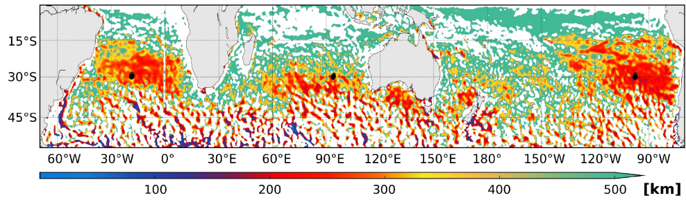
Figure 6: Characteristic length L_c (in km) over which the convergence and diffusion processes are balanced for the C-GLORS surface currents. The data were smoothed in space over distances of 1^\circ . The white color corresponds to positive divergence values. The black dots correspond to the centers of mass of the accumulation in each convergence zone for year 29 of the corresponding simulation of particle advection by the Ariane software (as defined in Figure 2).
