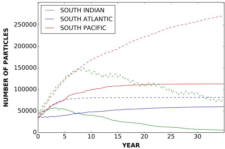
Figure 3: Time evolution of the number of particles in each convergence zone of the Southern Hemisphere when advected by C-GLORS surface currents only (dashed lines) or by the IOWAGA surface Stokes drift added to C-GLORS surface currents (plain lines). Beached particles (next to a land point) are excluded from the count. It should be noted that a much higher number of particles are blocked along the coast in regions with strong inshore currents when Stokes drift is added (67% totalling 610,000, compared to 20% totalling 182,000 without Stokes drift), hence reducing the total number of particles potentially trapped in convergence regions.
