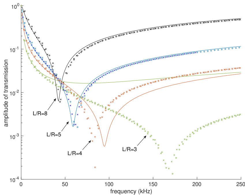
Figure 2. Comparison between the model (Equations (7), solid lines) and the numerical simulations by MST (Multel, crosses) and FEM (COMSOL, circles) for the transmission through arrays of R = 0.1 mm air bubbles in water with different lattice constants L .
