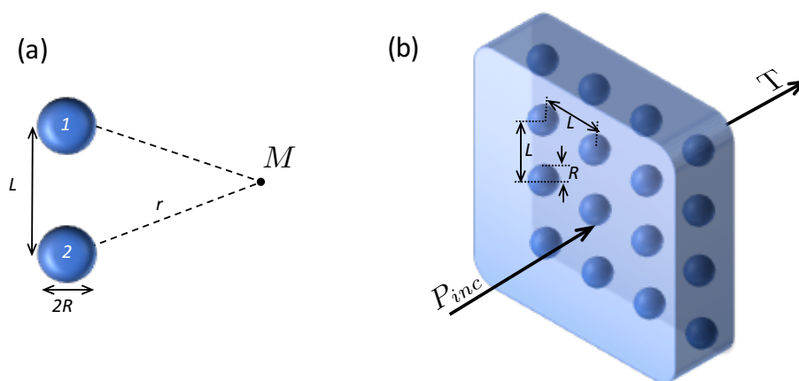
Figure 1. (a) A pair of R -radius bubbles, separated by a distance L . (b) An infinite array of R -radius bubbles, with a lattice distance L , excited by a plane wave with amplitude P_{inc} .
