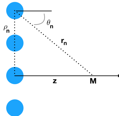
Figure A1. The pressure field generated by scatterer n at Point M is given by Equation (A2).
