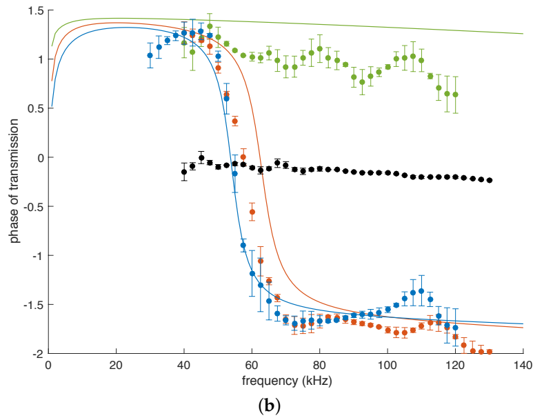
Figure 4. Amplitude (a) and phase (b) of the acoustic transmission through arrays of air bubbles in a yield-stress fluid (see Table 1 for the geometrical parameters of the samples). Black symbols show the result for the yield-stress fluid alone, without bubbles. Solid lines are the predictions of Equation (7).
