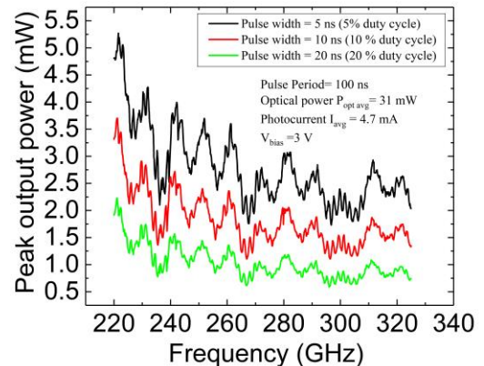
Fig. 2: Peak Output power as a function of frequency
