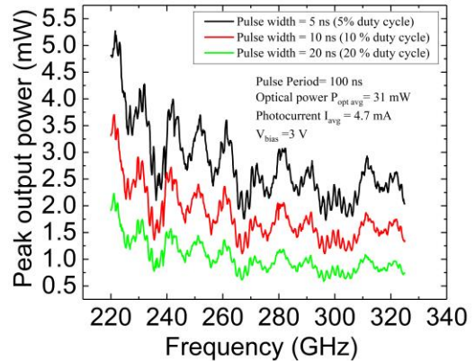
Fig. 2: Peak Output power as a function of frequency
