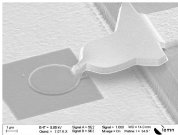
Fig. 1: SEM picture of a Fabry-Pérot cavity photoconductor coupled to a thin film microstrip line
