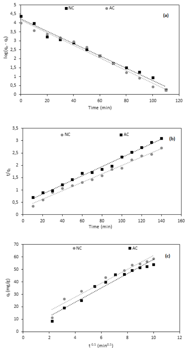
Fig. 10. Kinetics models of adsorption of the indigo blue on NC and AC: pseudo-first-order (a), pseudo-second-order (b), intra-particle diffusion (c).
