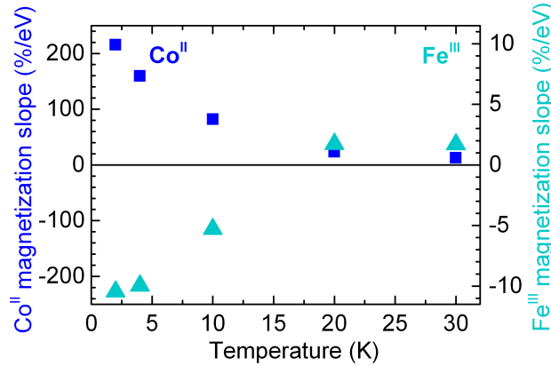
Figure 4: Slope at \mathbf{B} = 0 T for the \text{Fe}^{\text{III}} ( \blacktriangle ) and \text{Co}^{\text{II}} ( \blacksquare ) magnetization curves as a function of temperature obtained from XMCD detected magnetization curves (shown in S.I. section VII , Figure S9 ).
