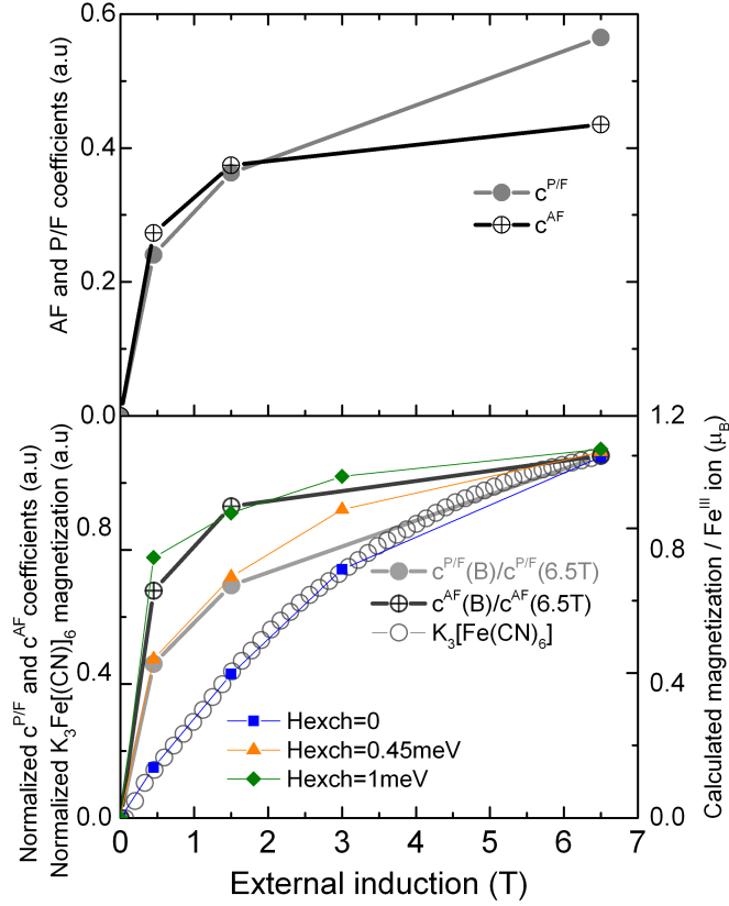
Figure 7: Coefficients c^{AF}(\mathbf{B}) (black line with \oplus ) and c^{P/F}(\mathbf{B}) (grey line with \bullet ) curves compared with K_3[Fe(CN)_6] XMCD detected magnetization curve ( \circ ) and with theoretical magnetization curves calculated with LFM model for Fe_{LS}^{III} ion with exchange magnetic energies equal to 0 ( \blacksquare ), 0.45 meV ( \blacktriangle ) and 1.0 meV ( \blacklozenge ).
