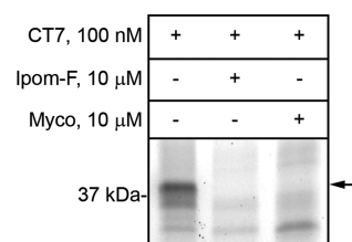
Figure 6. Sheep rough microsomes were preincubated with ipomoeassin F (Ipom-F) or mycolactone (Myco) at 10 \mu\text{M} . Subsequently 100 nM photocotransin CT7 was added and samples were photolyzed. The covalent CT7/Sec61 \alpha adduct was detected using click chemistry to install a rhodamine-azide reporter and in-gel fluorescent scanning.
