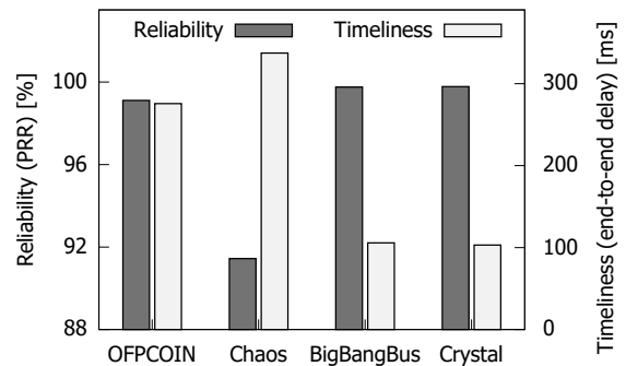
Fig. 4: Exemplary results obtained during the EWSN 2018 dependability competition, comparing the reliability and timeliness of different IoT protocols.
