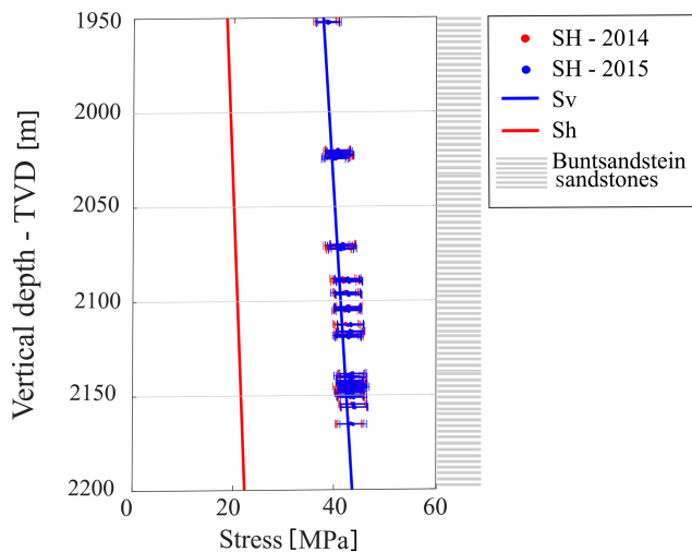
Figure 17. In situ stress components S_h , S_v and S_H (MPa) in the deviated well GRT-2. S_H stresses are inverted using a Mohr–Coulomb failure criterion and represented as a function of vertical depth (TVD) for the images acquired in 2014 and 2015. Error bars are calculated considering the errors on the measurements of the breakout widths, on the elastic parameters, and on the S_h and S_v trends. The right column illustrates the lithological unit retained in the model.
