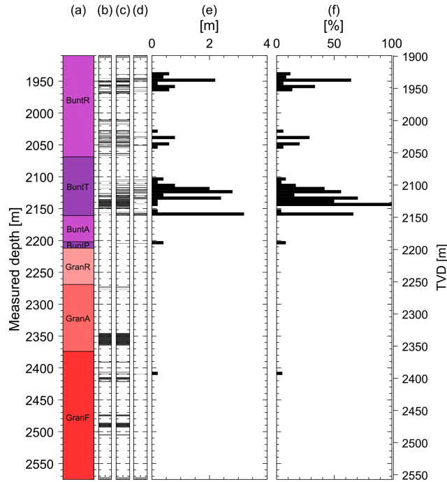
Figure 8. Development of breakouts along the GRT-1 borehole between 2012 and 2013. (a) Simplified lithologies along the GRT-1 borehole as a function of measured depth (MD) or vertical depth (TVD). BuntR stands for Couches de Rehberg, BuntT for Couches de Trifels, BuntA for Annweiler sandstone, BuntP for Permian layers older than Annweiler sandstone, GranR for rubefied granites, GranA for hydrothermally altered granite and GranF for low altered granite. The major fault zone crossing GRT-1 at 2368 m is represented as a black band. (b) Breakout positions in GRT-1 in 2012. (c) Breakout positions in GRT-1 in 2013. (d) Intervals at which breakouts are present in 2013 but not in 2012. (e) Breakout length increase (m) along the borehole between 2012 and 2013 in 5 m bins. (f) Fraction (%) of wellbore length that was free of a breakout in 2012 but presents a breakout on the 2013 image, computed in 5 m bins.
