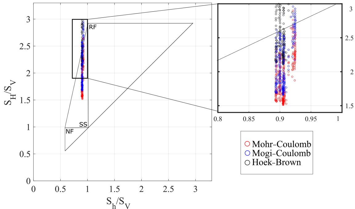
Figure 16. Normalized stress polygon defining stress states ( S_H/S_V , S_h/S_V ) at a depth of 2500 m in GRT-1, according to a Coulomb law with a coefficient of friction \mu = 1 . The borders of the polygon correspond to an active fault situation. RF – reverse faulting, SS – strike-slip regime and NF – normal faulting refer to Anderson’s faulting regimes. The plot includes stresses ( S_H/S_V – S_h/S_V ) calculated from the image of GRT-1 from 2013 for three different failure criteria (circles in color).
