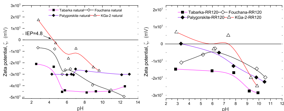
Fig. 3. Variation of the zeta potential, \zeta , of the various clay aqueous dispersions with the aqueous phase pH, in the absence and in the presence of RR 120 dye molecules.
